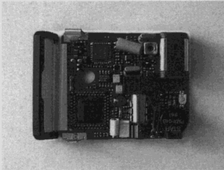
(SOLDER SIDE)
