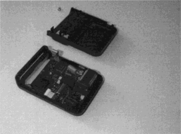
REAR VIEW OF THE EUT (REAR COVER REMOVED)
