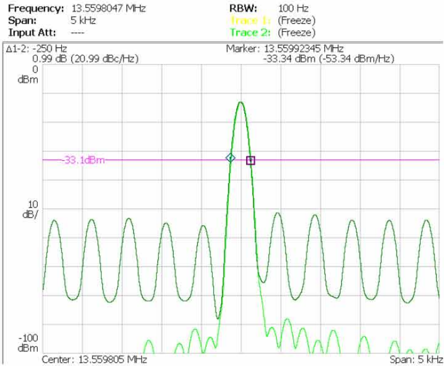
Figure A-5: Test result of EUT1 at test set. RFID02
