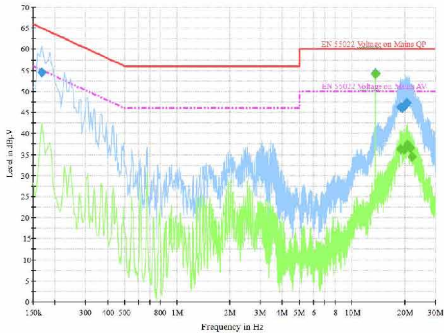
Figure A-6: Test result of EUT1 at test set. RFID01
