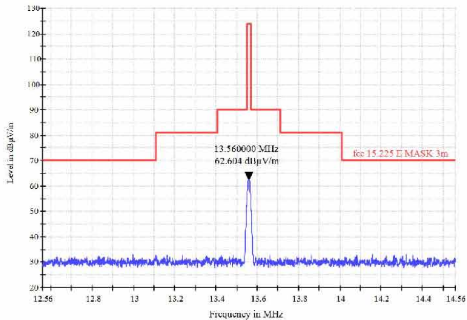
Figure A-1: Set. RFID01
