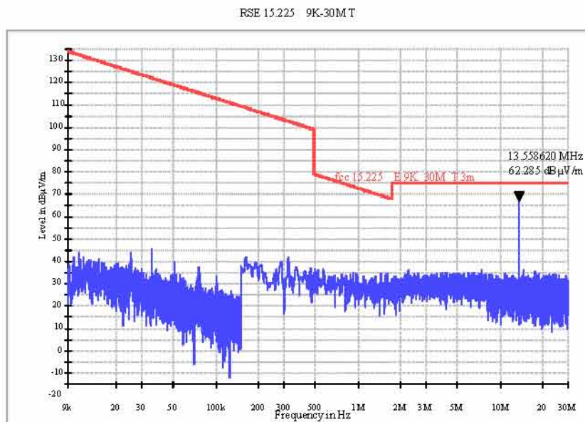
Figure A-2: Set. RFID01
