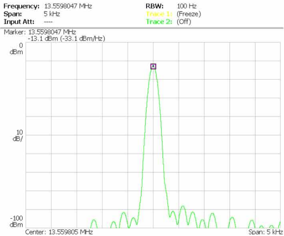
Figure A-4: Test result of EUT1 at test set. RFID02
