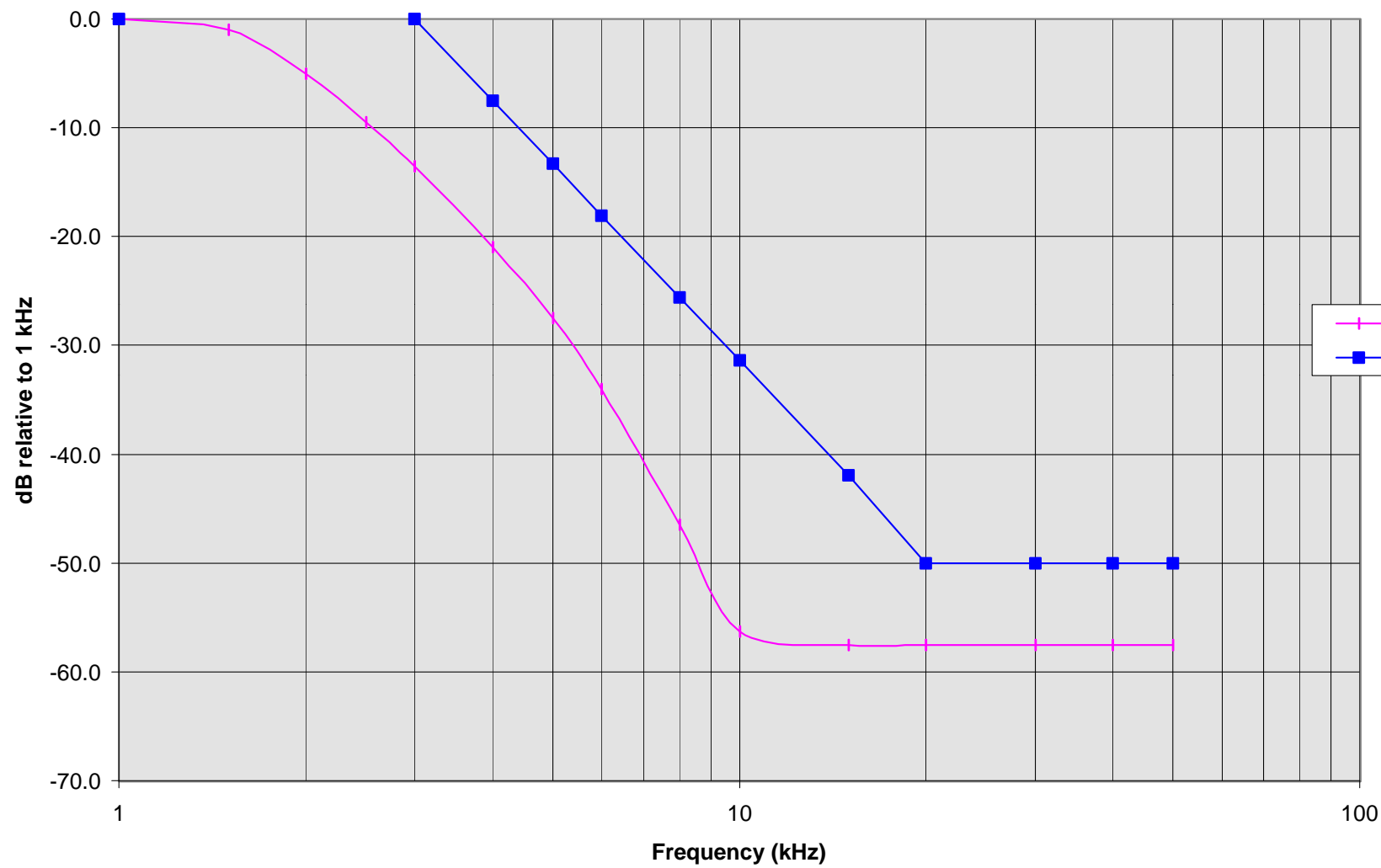
Audio Low Pass Filter Response
