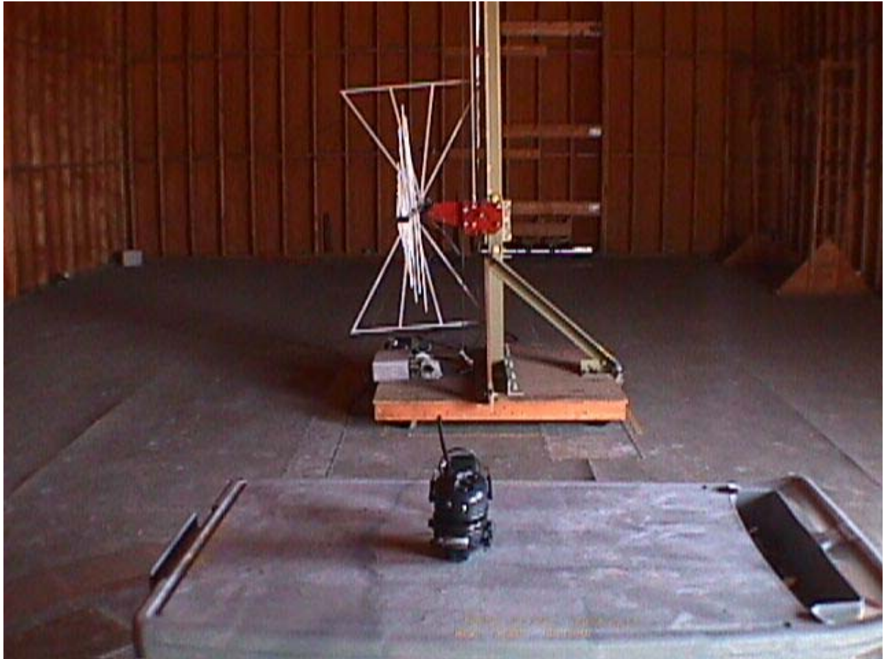
Radiated Emissions at 3 Meters Distance Orthogonal Position # 2
