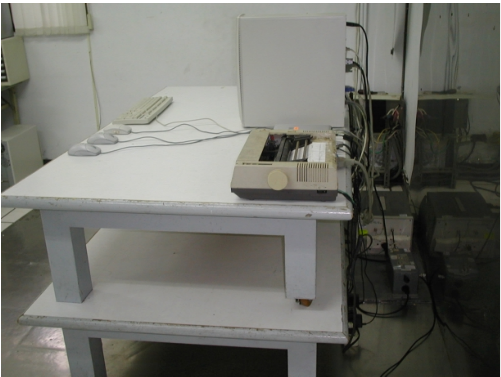
Set-up Photo ( Conduction Back )
