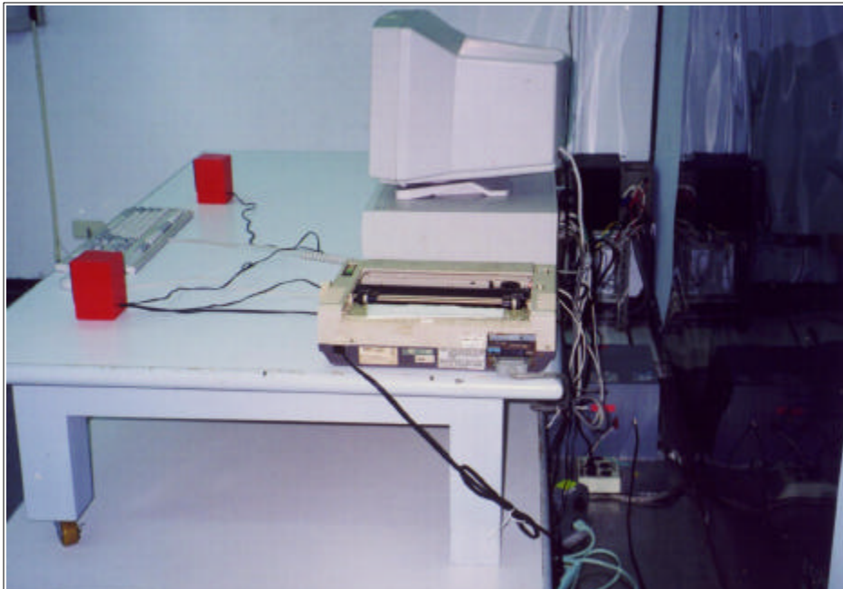
Conducted Emission Setup Photos (Worst Emission Position)
