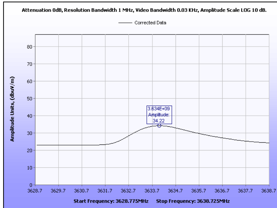
Plot 2. Radiated Spurious Emissions, 4 th Harmonic, Average, 9.6kbps
