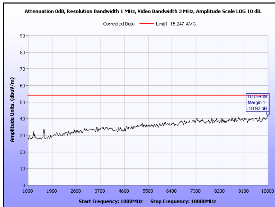
Plot 17. Receiver Spurious Emission, 1 GHz – 10 GHz
