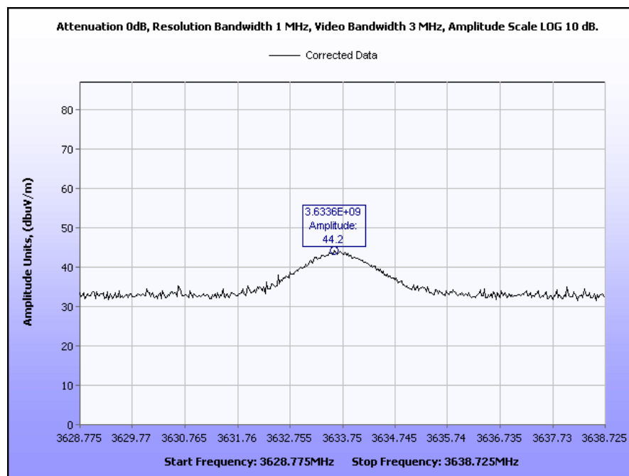
Plot 3. Radiated Spurious Emissions, 4 th Harmonic, Peak, 9.6kbps
