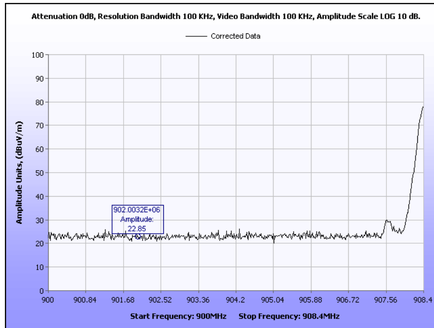
Plot 12. Radiated Band Edge, Low Channel, 9.6 kbps
