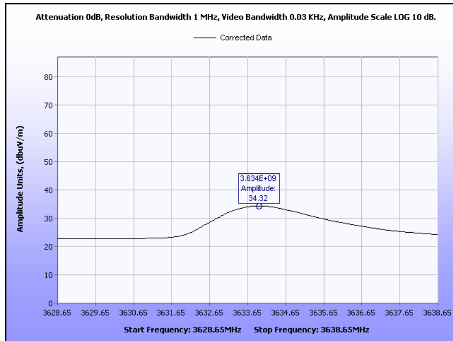
Plot 4. Radiated Spurious Emissions, 4 th Harmonic, Average, 40kbps
