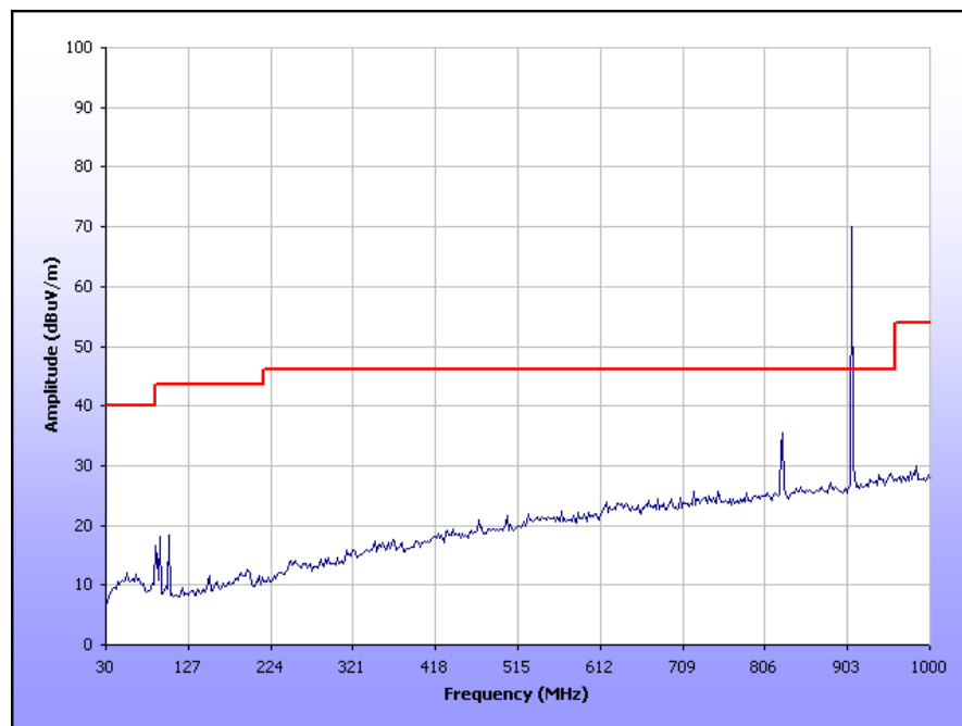
Plot 9. Radiated Spurious Emissions, 30 MHz – 1 GHz, 40kbps
