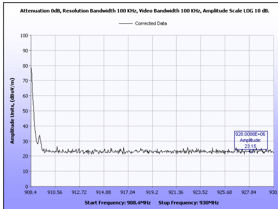
Plot 15. Radiated Band Edge, High Channel, 40 kbps
