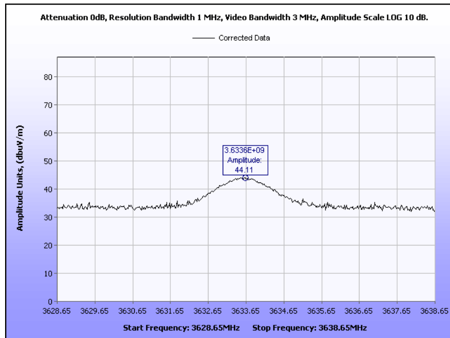
Plot 5. Radiated Spurious Emissions, 4 th Harmonic, Peak, 40kbps
