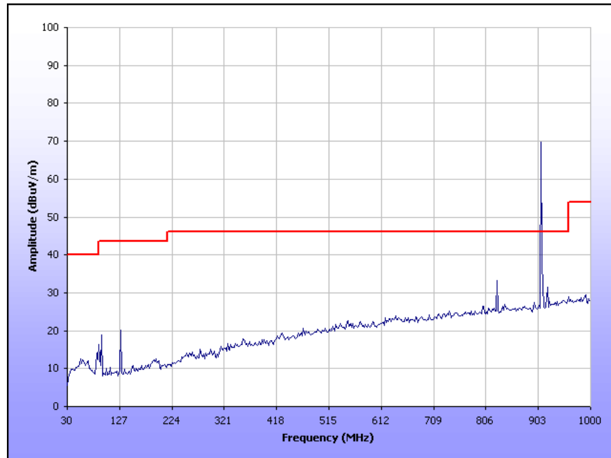
Plot 8. Radiated Spurious Emissions, 30 MHz – 1 GHz, 9.6kbps
