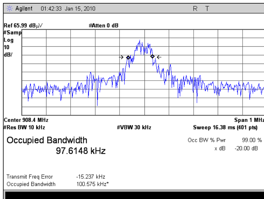
Plot 6. Occupied Bandwidth, 99% Bandwidth, 9.6 kbps
