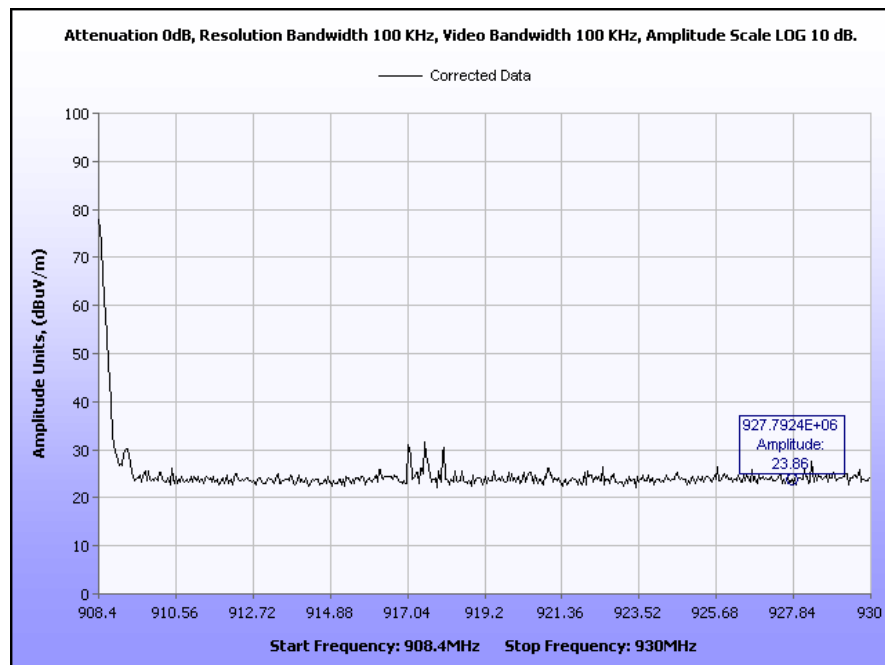
Plot 13. Radiated Band Edge, High Channel, 9.6 kbps
