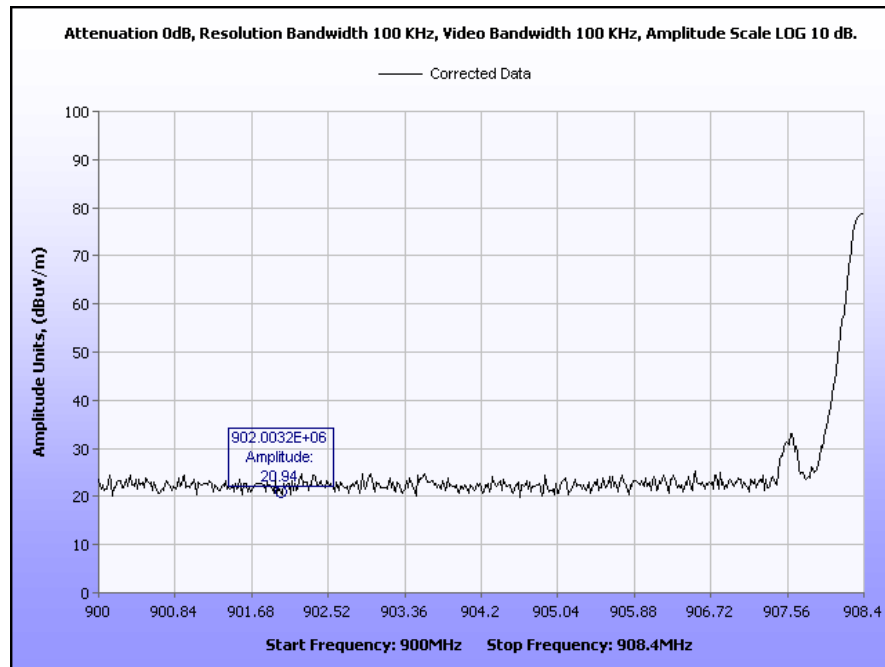
Plot 14. Radiated Band Edge, Low Channel, 40 kbps
