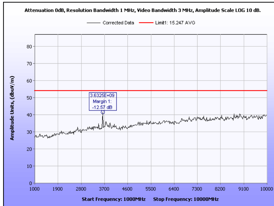
Plot 10. Radiated Spurious Emissions, 1 GHz – 10 GHz, 9.6kbps
