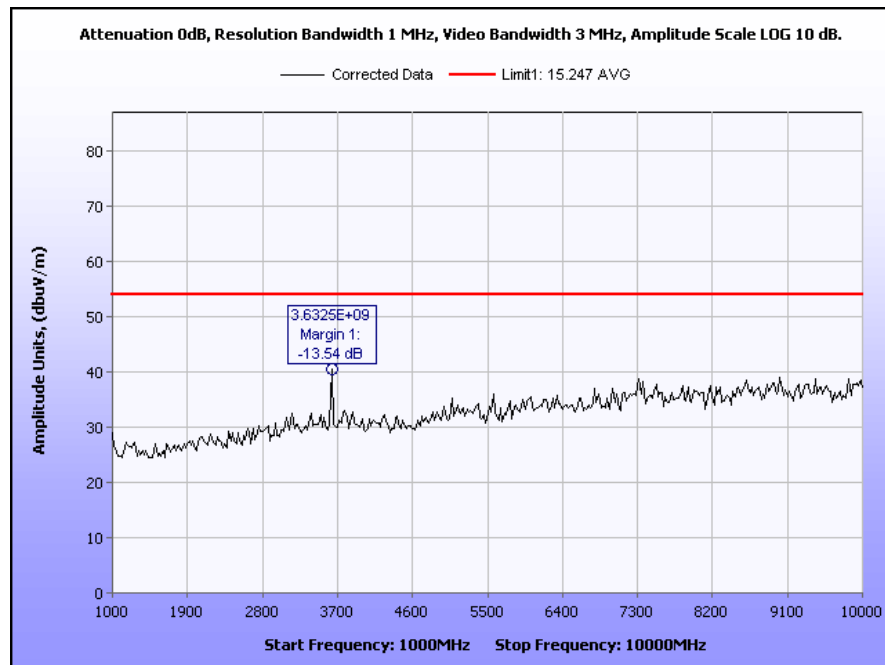
Plot 11. Radiated Spurious Emissions, 1 GHz – 10 GHz, 40kbps
