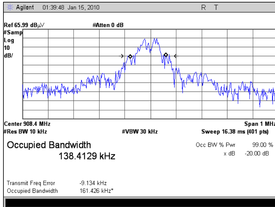
Plot 7. Occupied Bandwidth, 99% Bandwidth, 40 kbps
