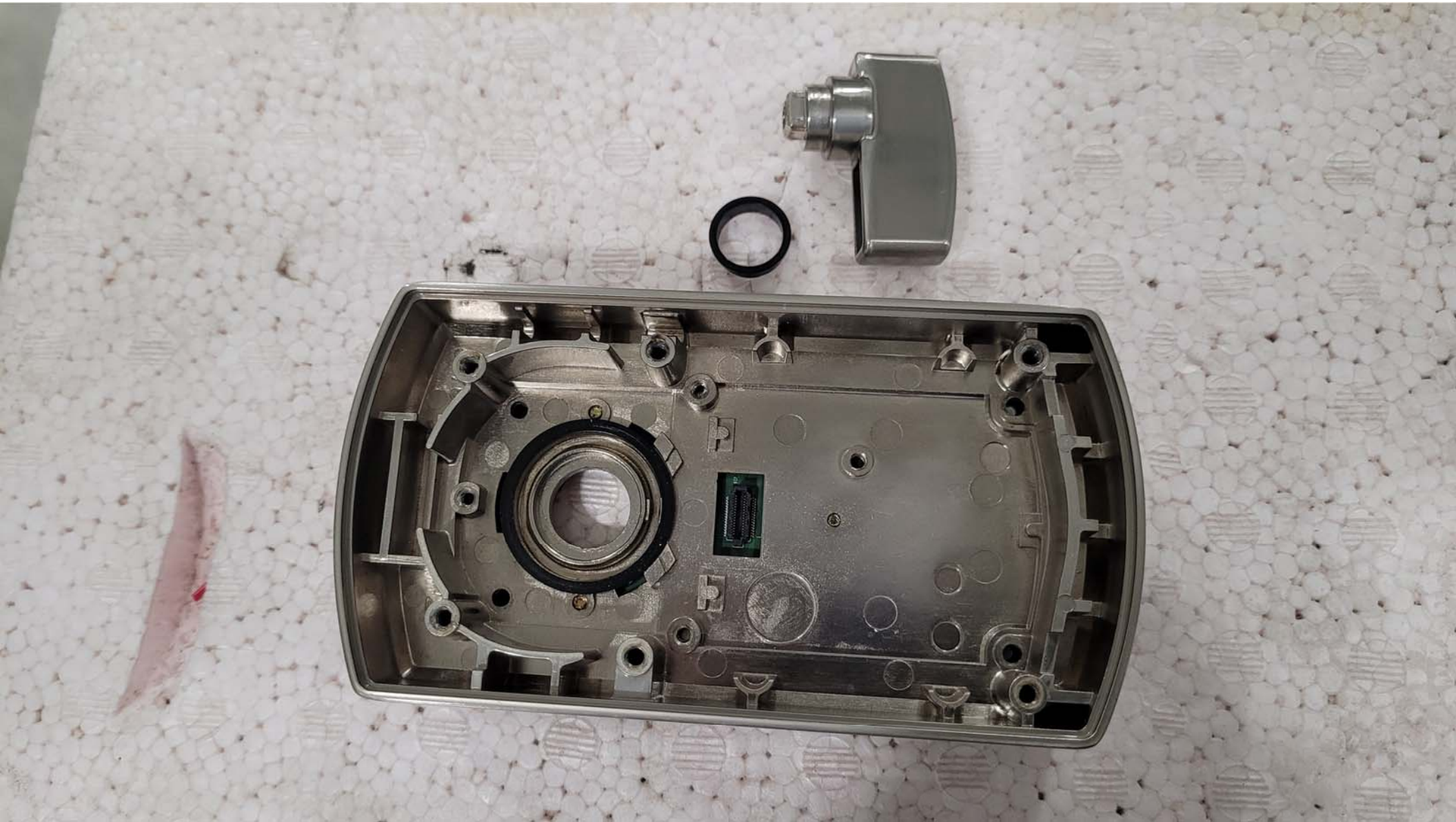
Inside View of the EUT - View #5
