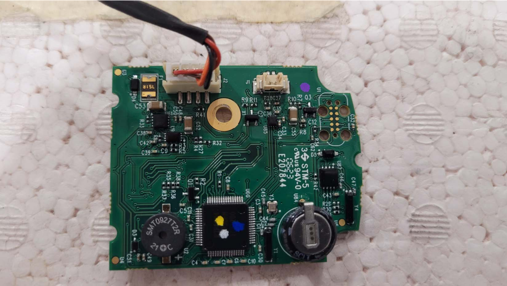
Top View of the Main PCB - View #1
