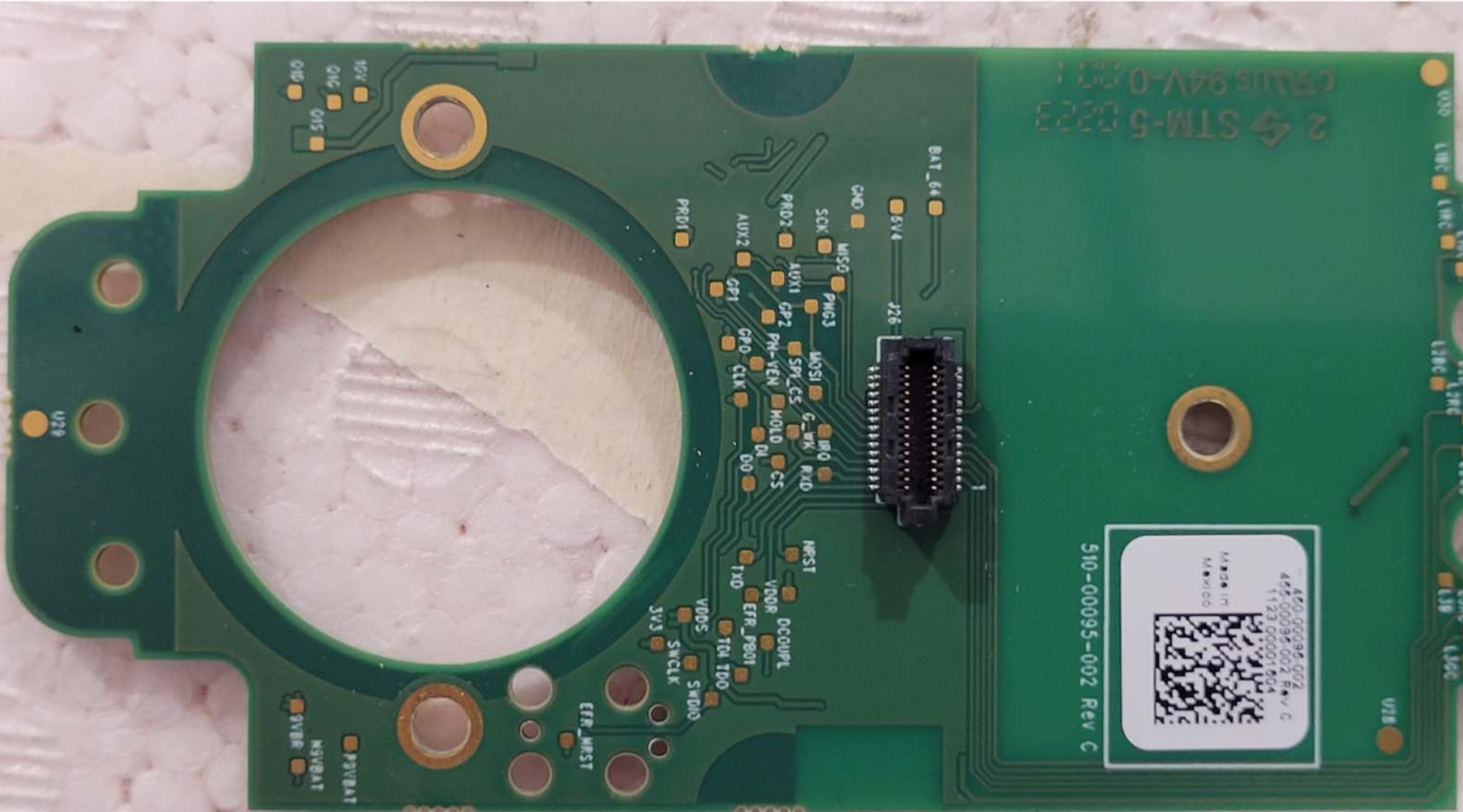
Bottom View of the RFID PCB for the EUT - View #1
