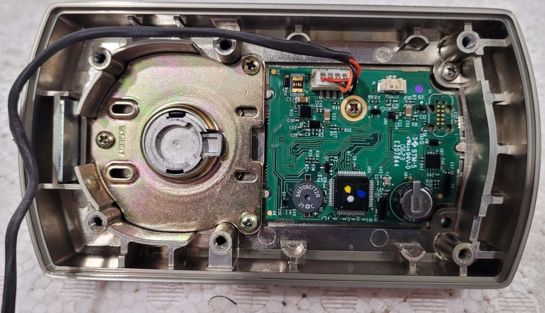
Inside View of the EUT - View #4
