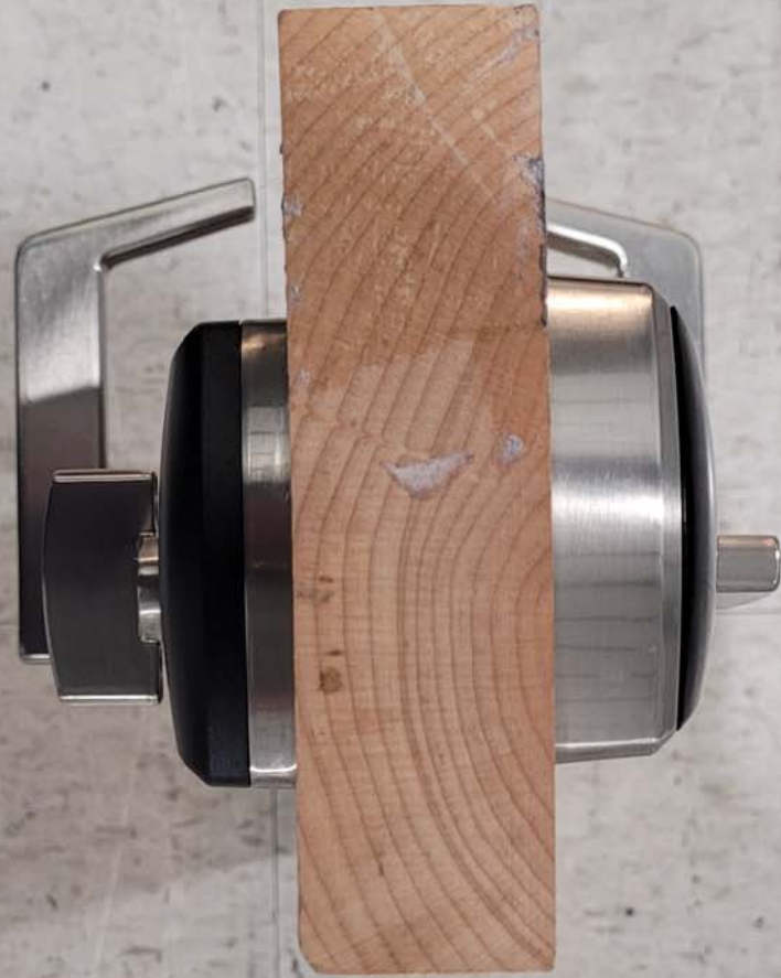
Top View of the EUT with 4.5 Inch Interconnect Enclosure
