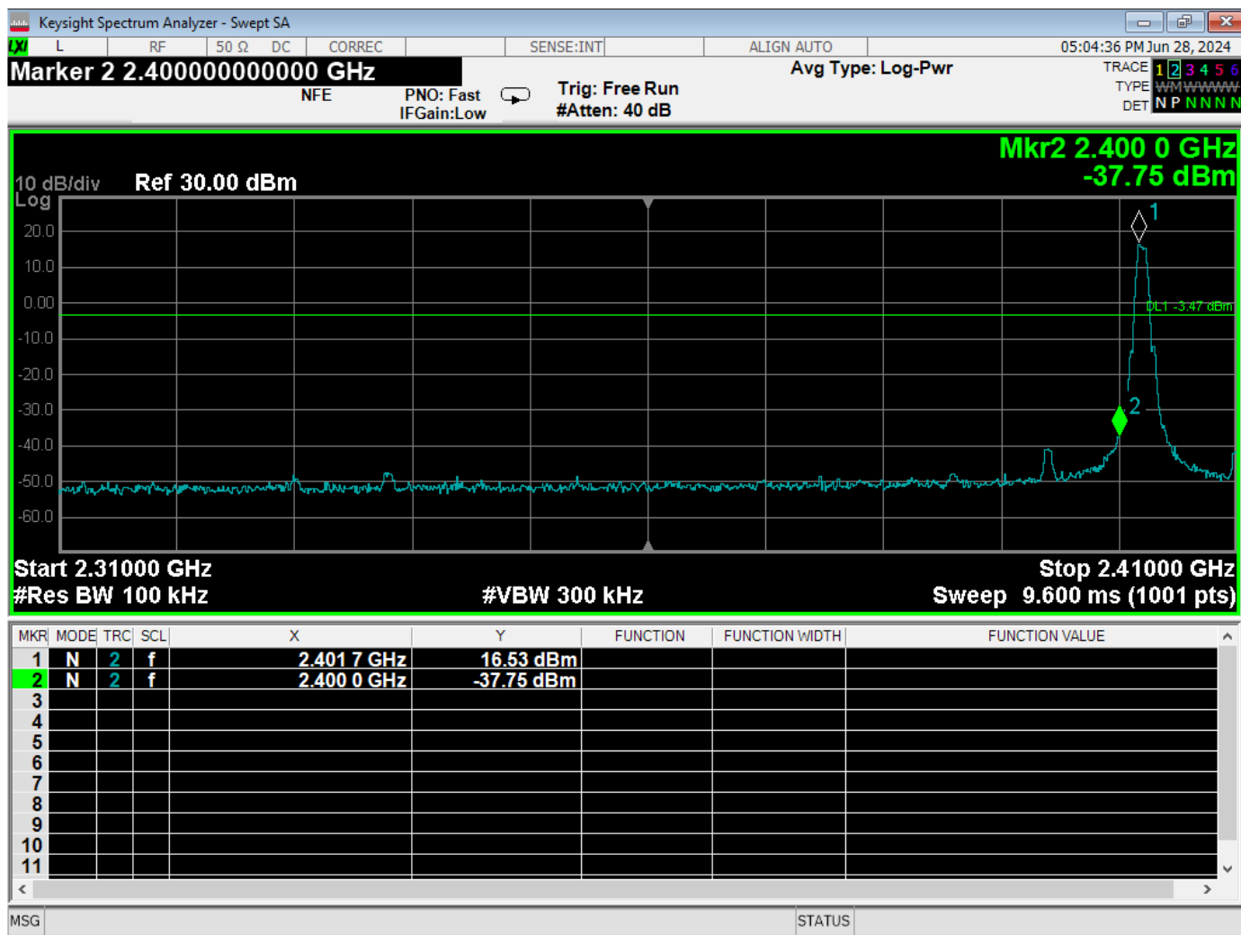
Band Edge – BLE Mode – Nordic – Low Channel – at 2400 MHz – Conducted Measurement
