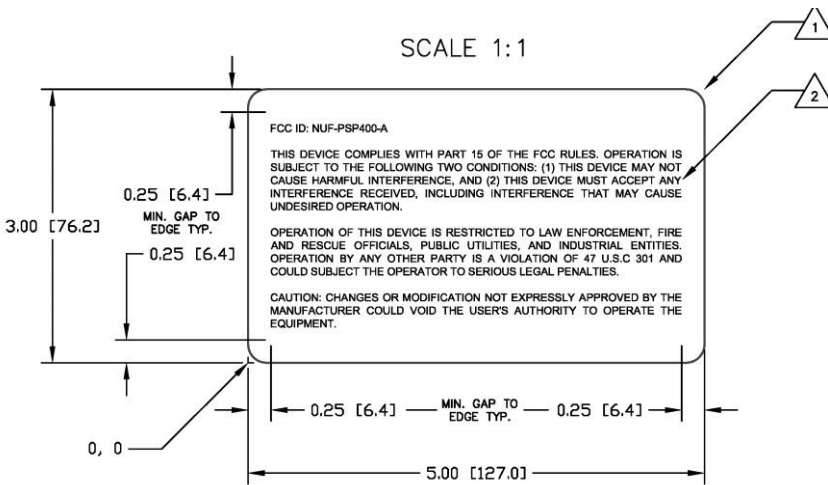
Fig. 16: Label with FCC ID number
