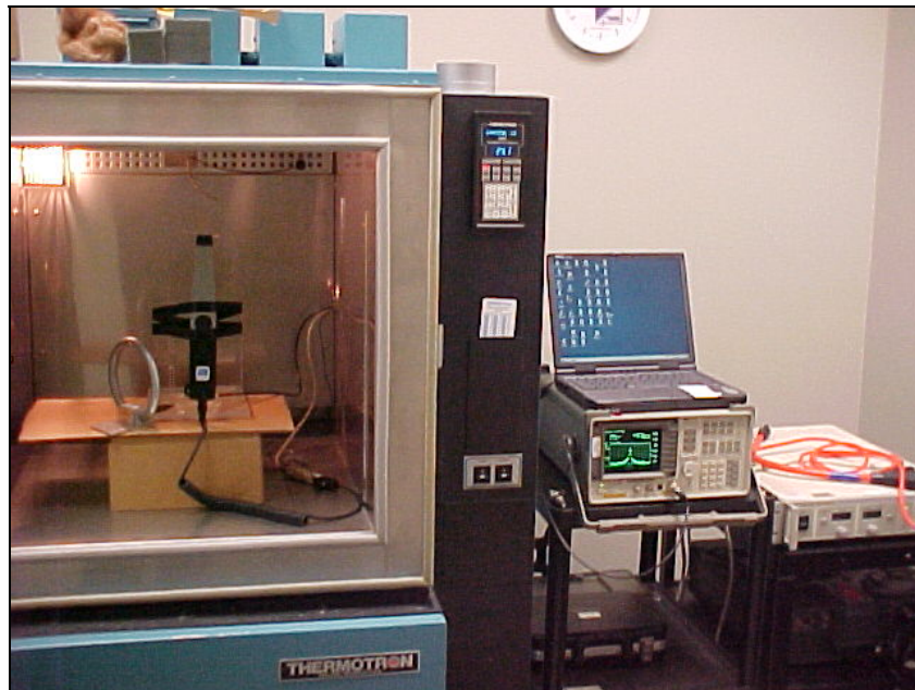
View of the EUT during Frequency Stability Testing
