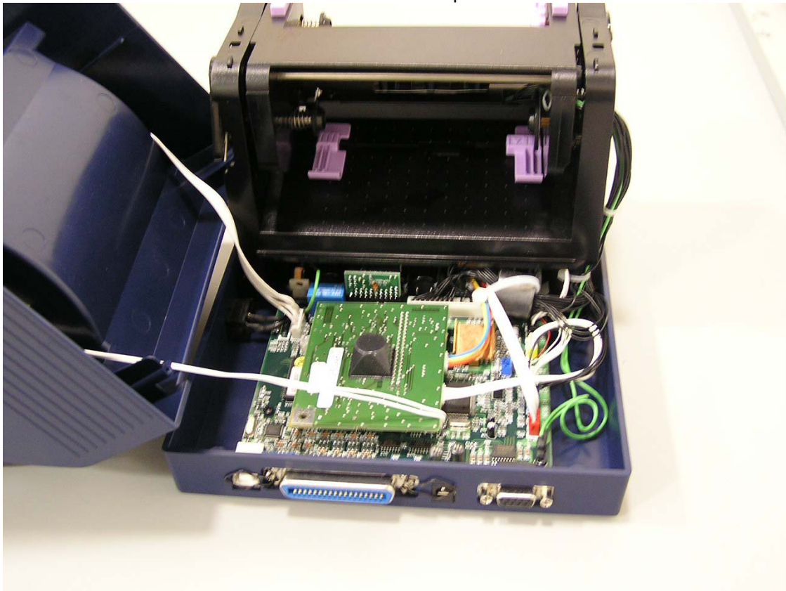
Antenna inside cover
