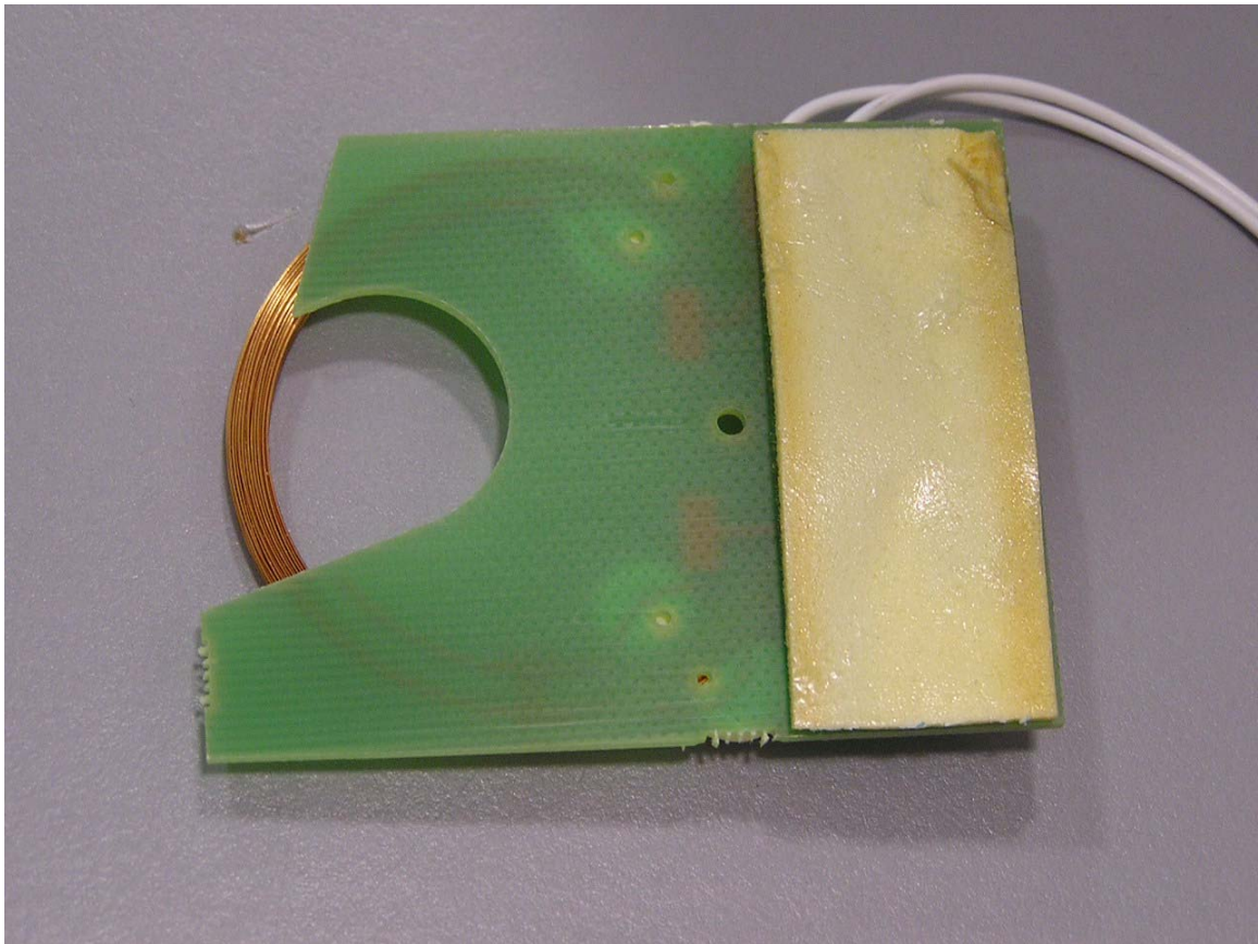
Antenna PWB front
