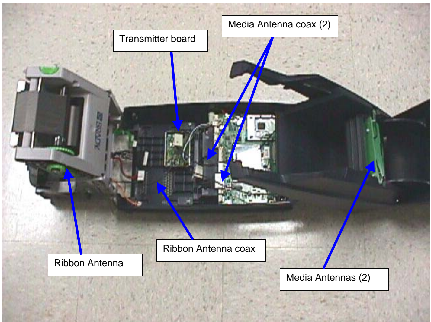
Figure 1 -- Overview of Antenna and Transmitter Board Locations in Printer
