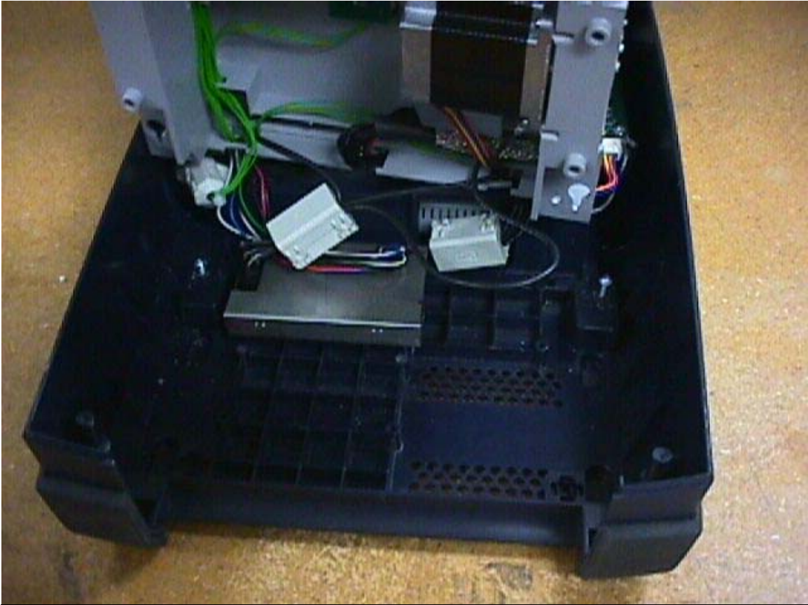
Figure 10 -- Internal view, Brady Daughter Card (BDC) in metal enclosure
