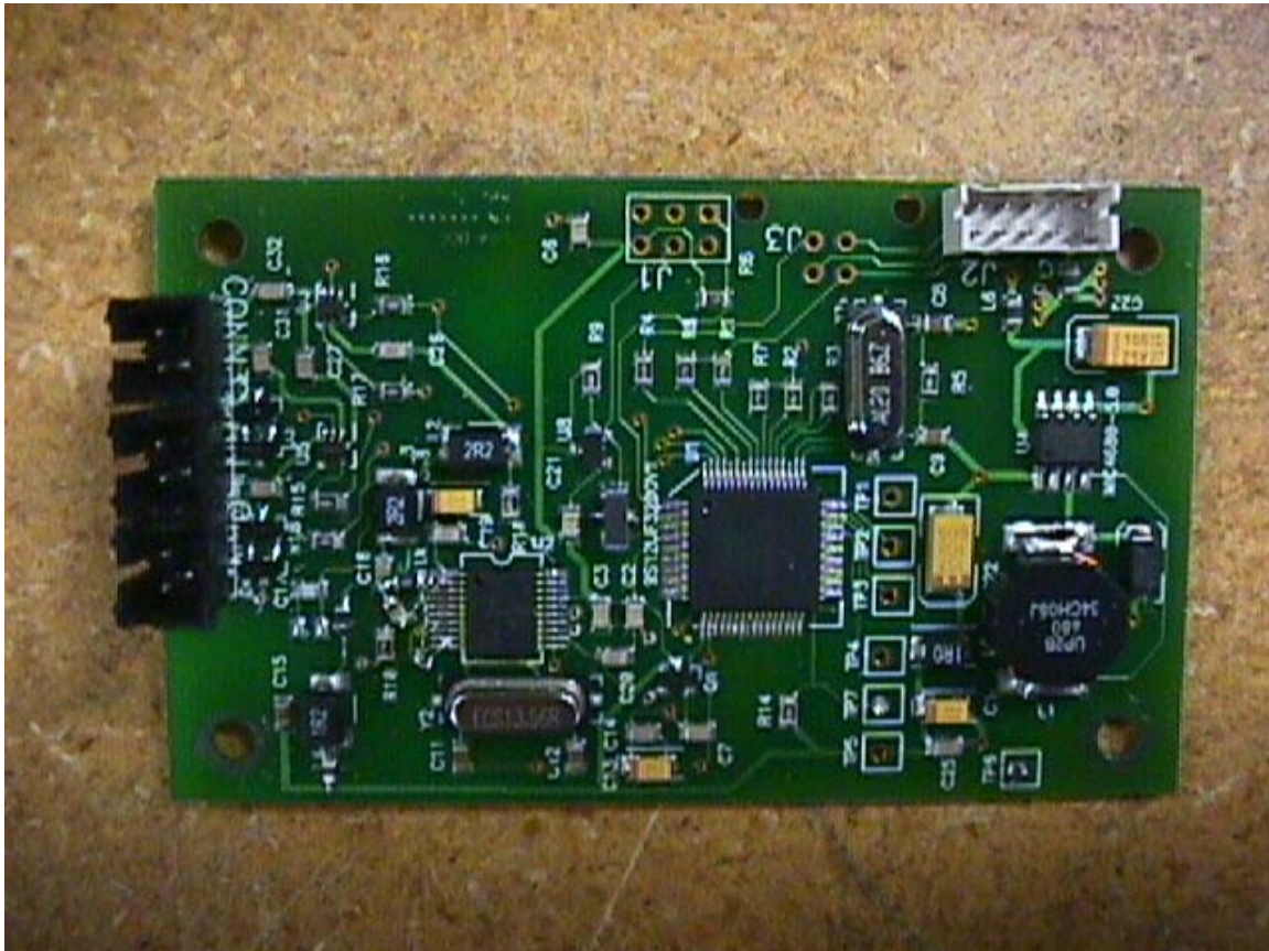
Figure 12 -- Internal view, BDC - top
