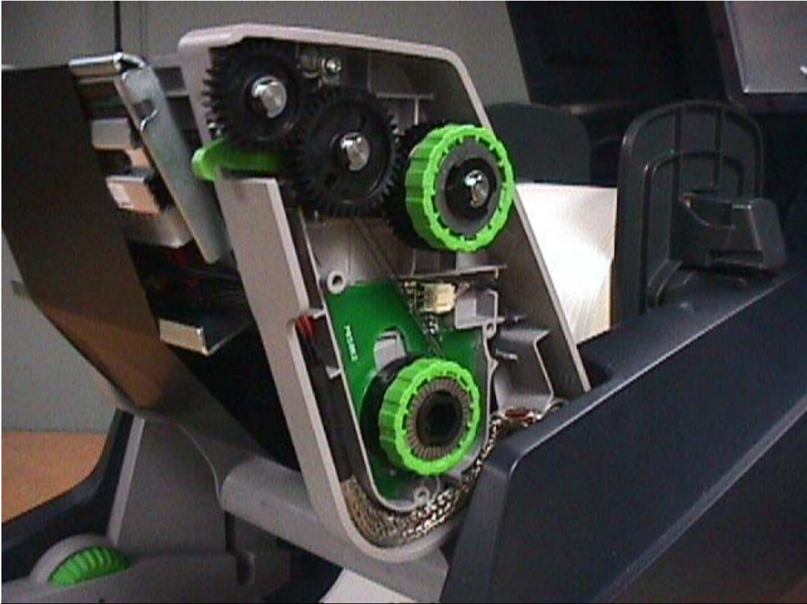
Figure 2 -- Internal view, ribbon antenna
