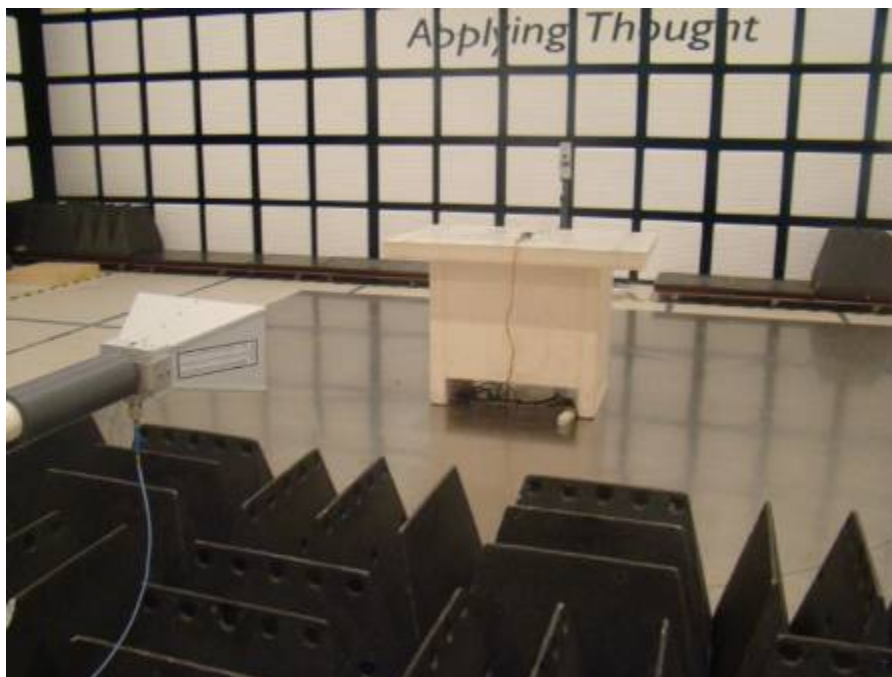
Figure 3: Test setup for Radiated Emission (Vertical) – 1GHz to 18GHz
