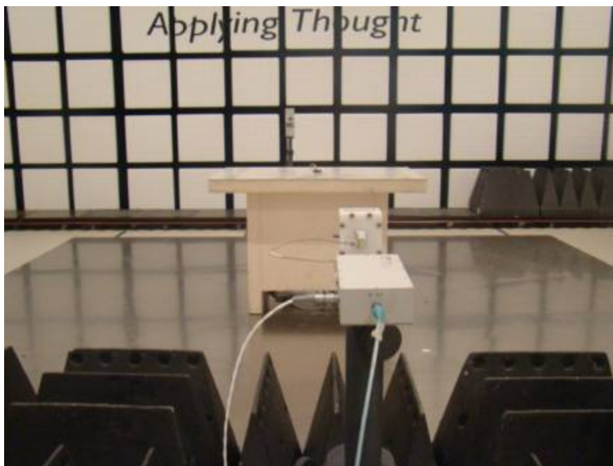
Figure 5: Test setup for Radiated Emission (Horizontal) – 18GHz to 25GHz
