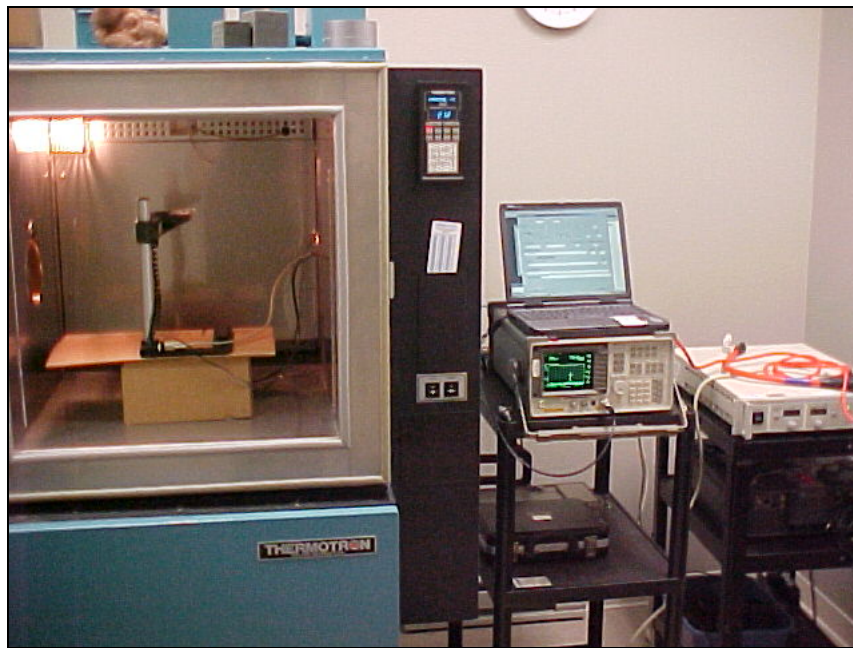
View of the EUT during the Frequency Stability testing
