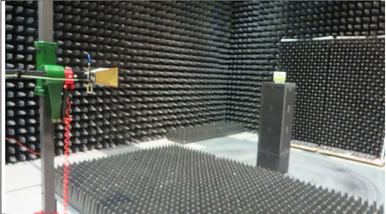
Description: Radiated Emission Setup
