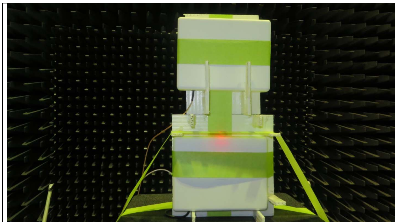
Description Unit with External Antenna mounted above
