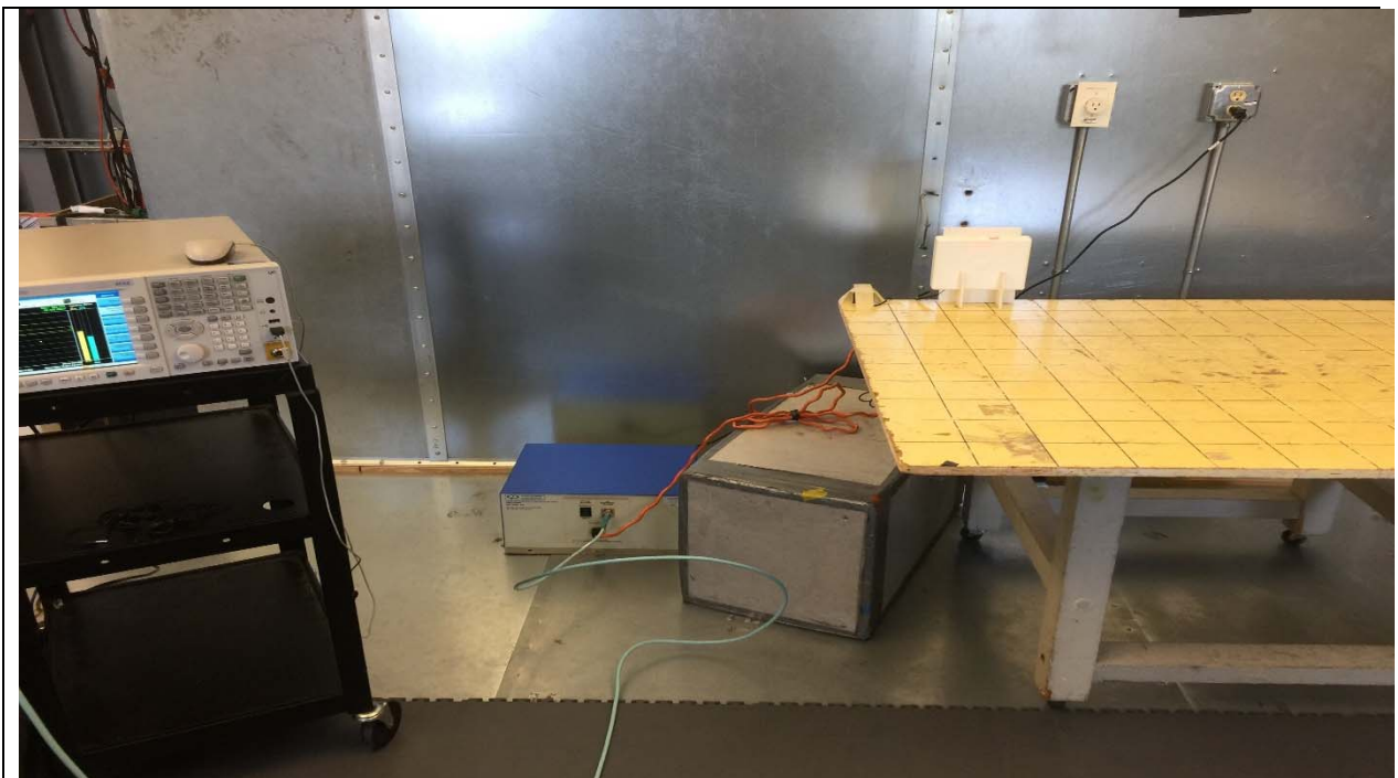
Description: Conducted Emission Setup
