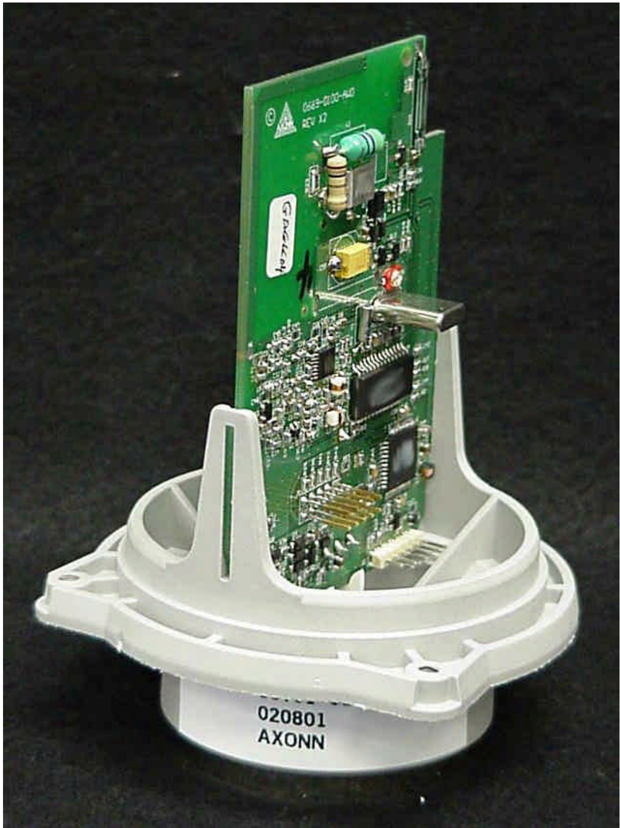
Photo 5. EUT, Front View Cover Removed
