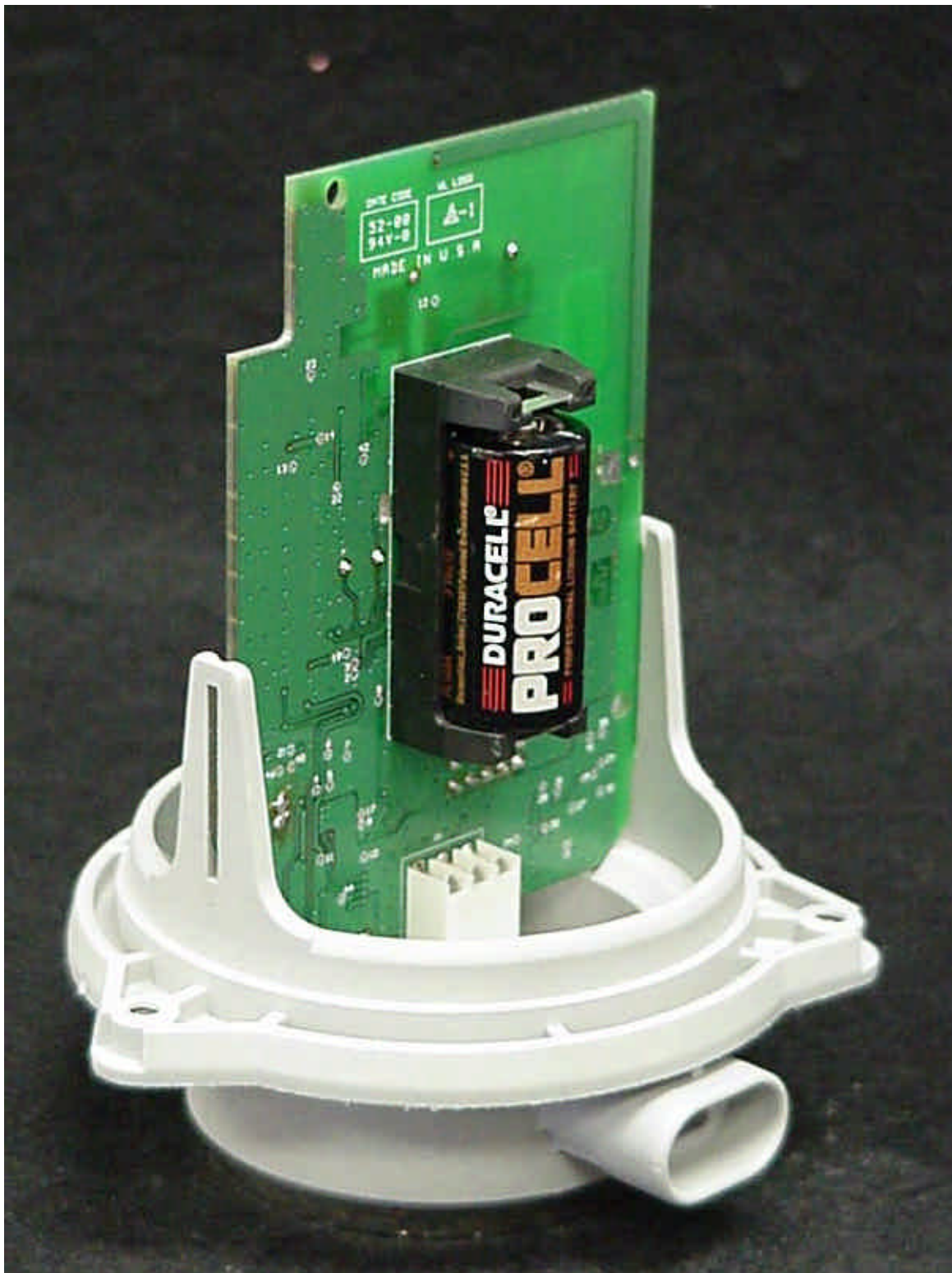
Photo 6. EUT, Rear View Cover Removed
