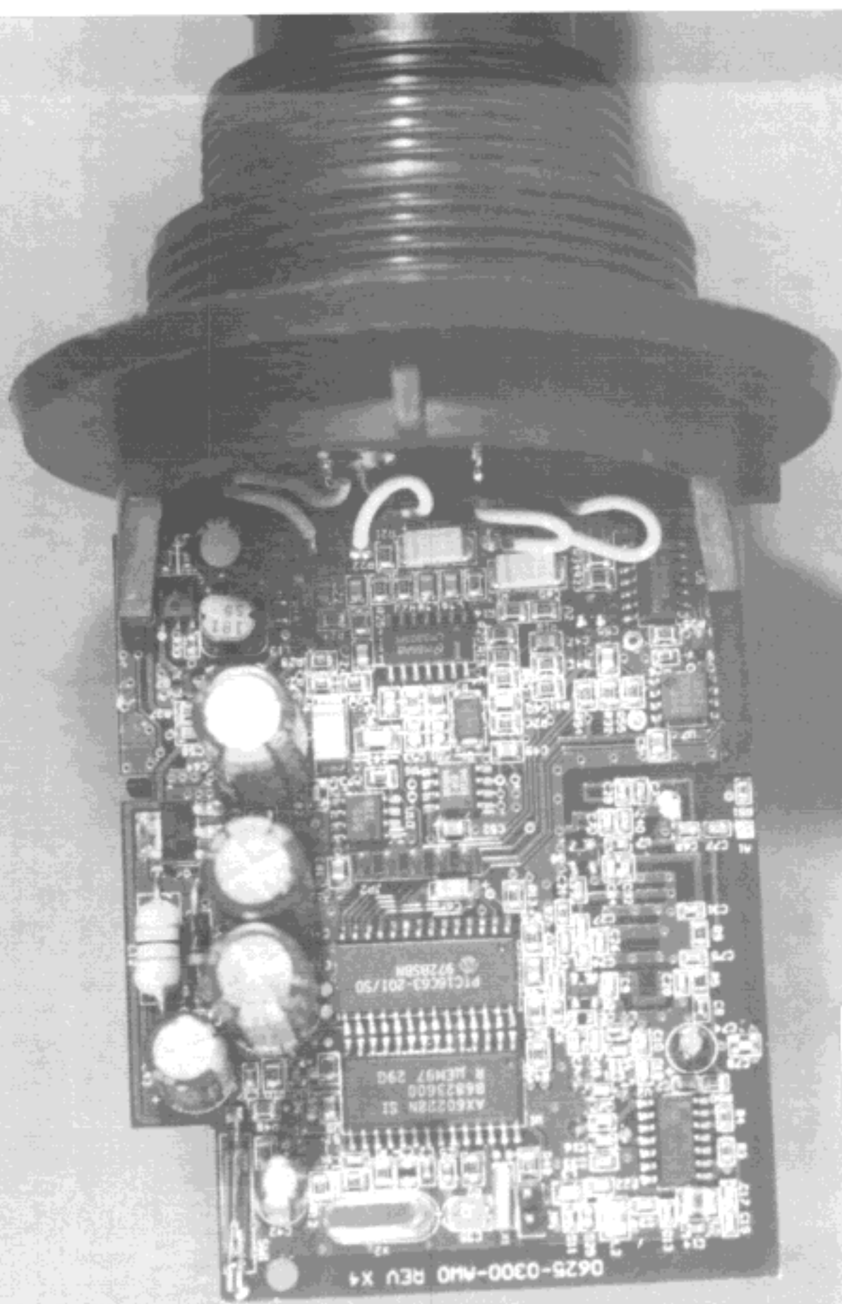
Photograph 4.2: Printed Circuit Board, Top View
