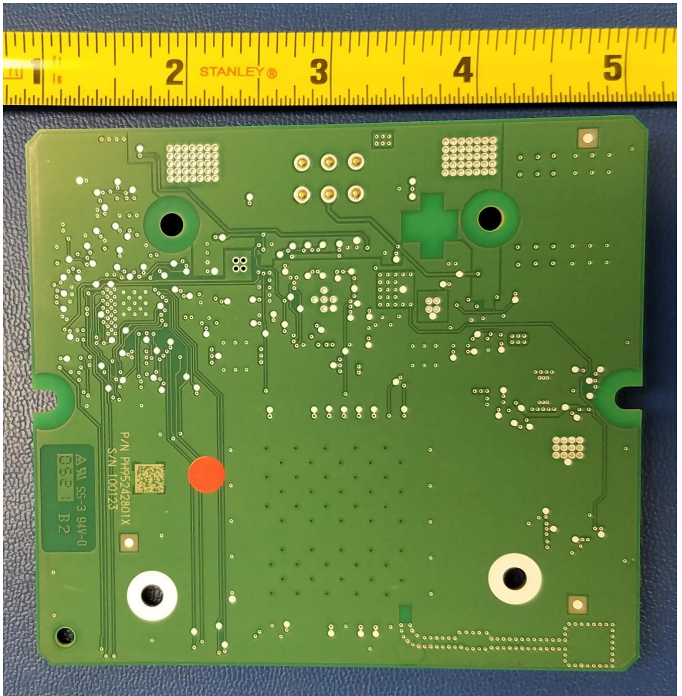
Figure 6: PCBA Bottom
