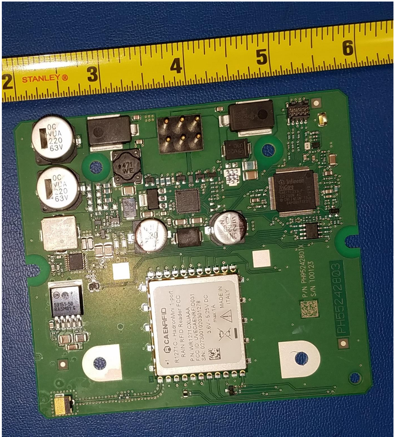
Figure 5: PCBA Top
