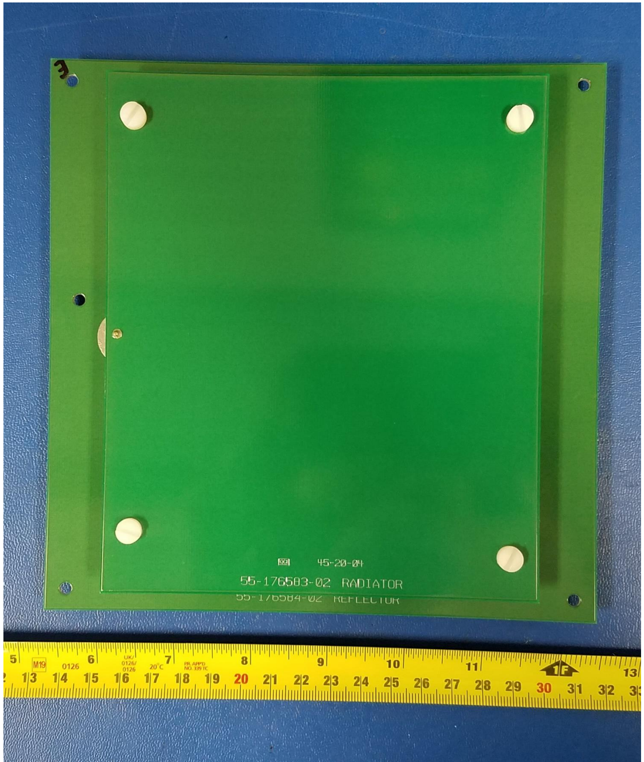
Figure 3: Antenna Top
