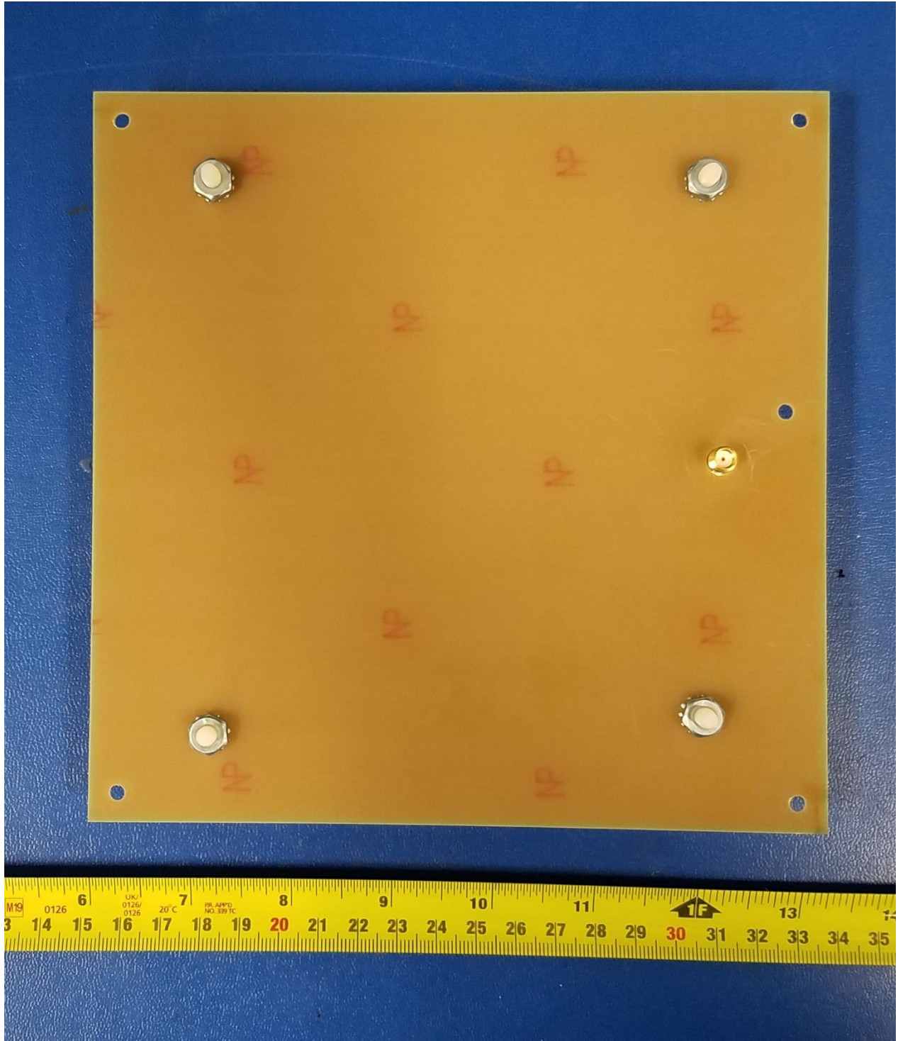
Figure 4: Antenna Bottom
