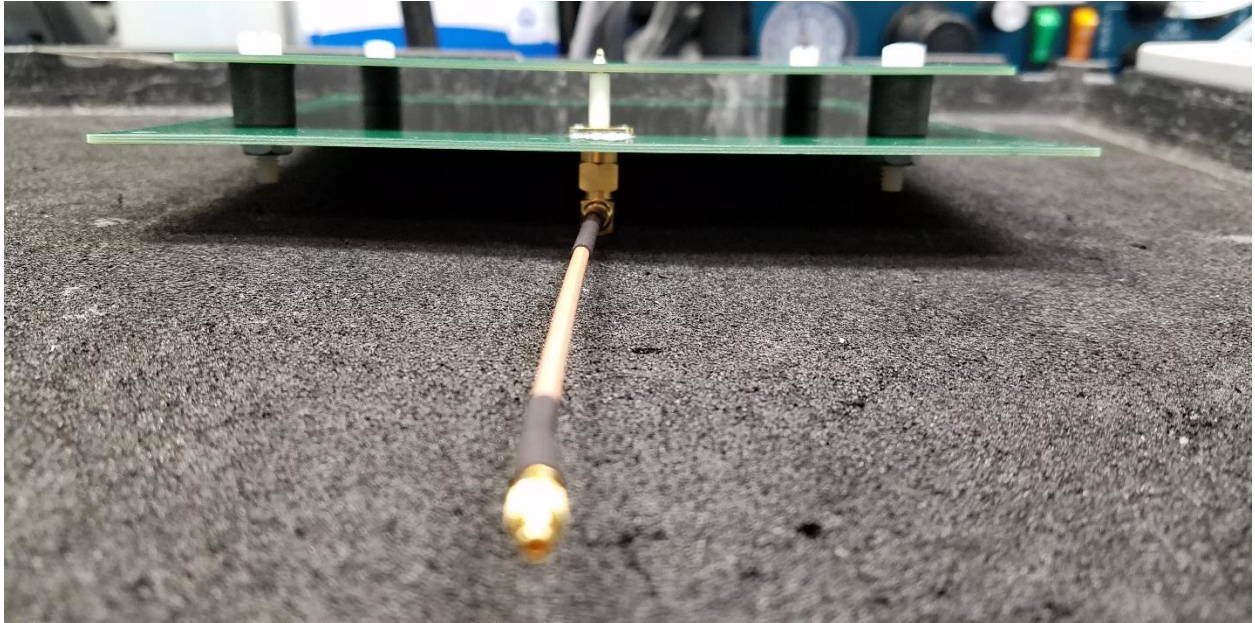
Figure 7: Antenna Front
