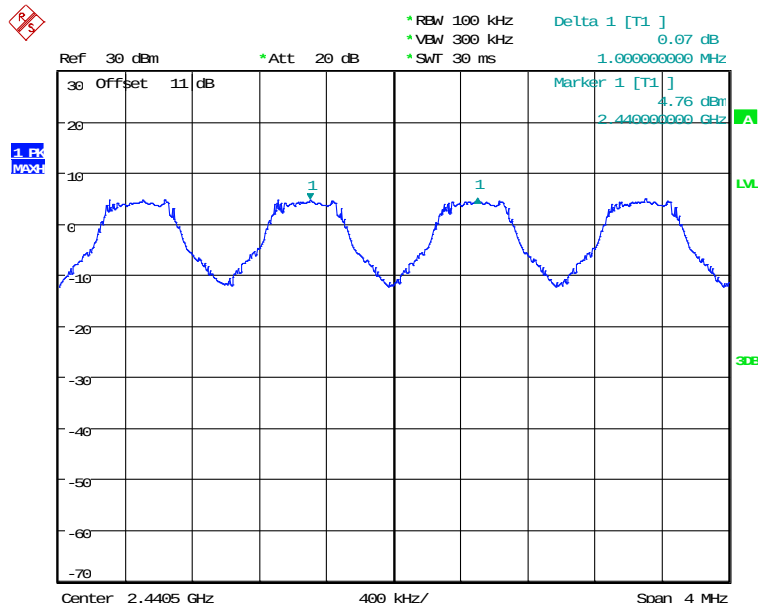
FREQUENCY SEPARATION CH39 Date: 20.JUN.2024 15:13:53
