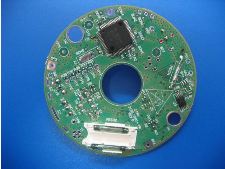
Photograph No.4 ETMW water reader PCB printed side
