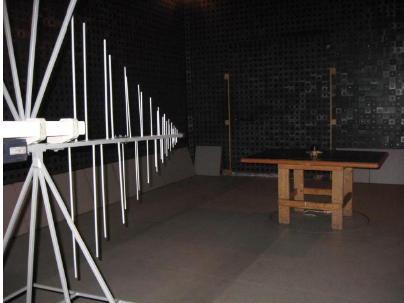
Photograph No.2 Setup for carrier field strength, power spectral density and spurious emission measurements in the anechoic chamber from 30 to 1000 MHz
