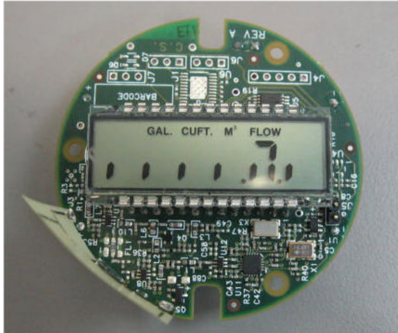
Photograph No.2 DTMW LCD water reader PCB top view
