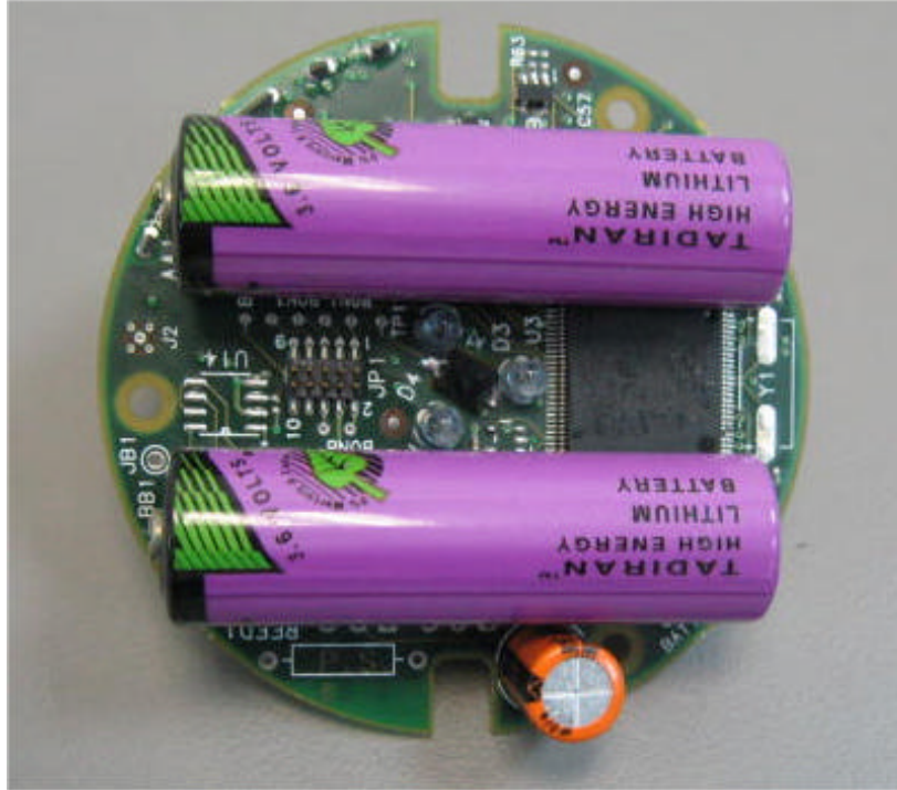
Photograph No.3 DTMW LCD water reader PCB second side view
