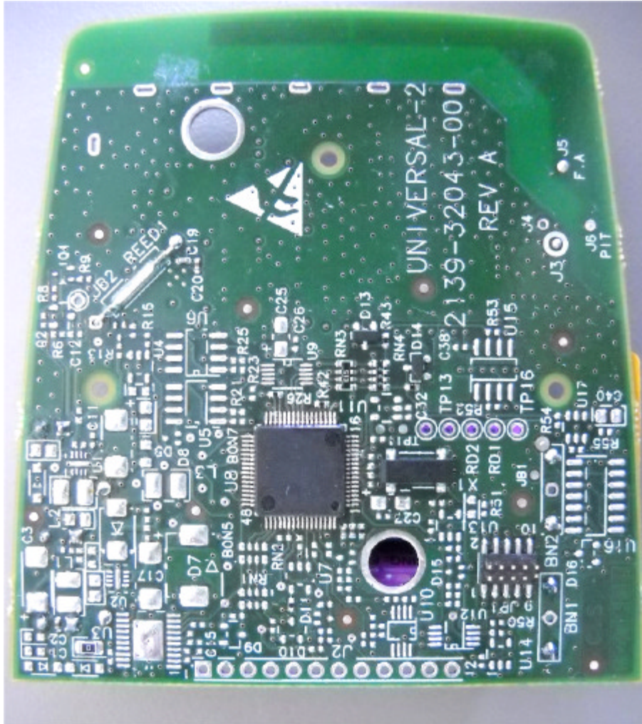
Photograph No.2 Water meter "Universal 2" PCB second side view
