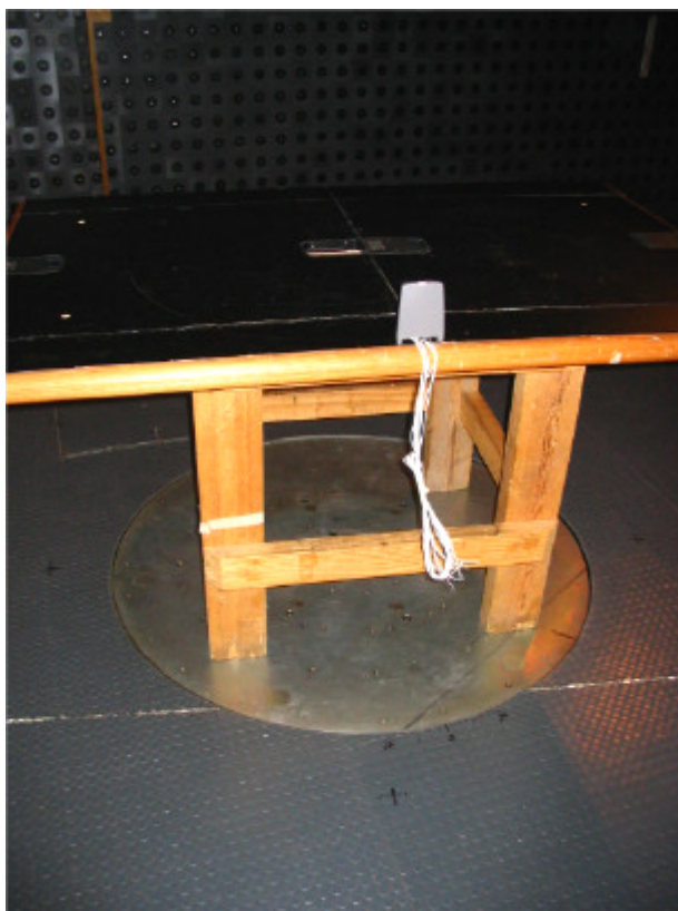
Photograph No.6 Setup for radiated emission measurements according to §15.109, close view
