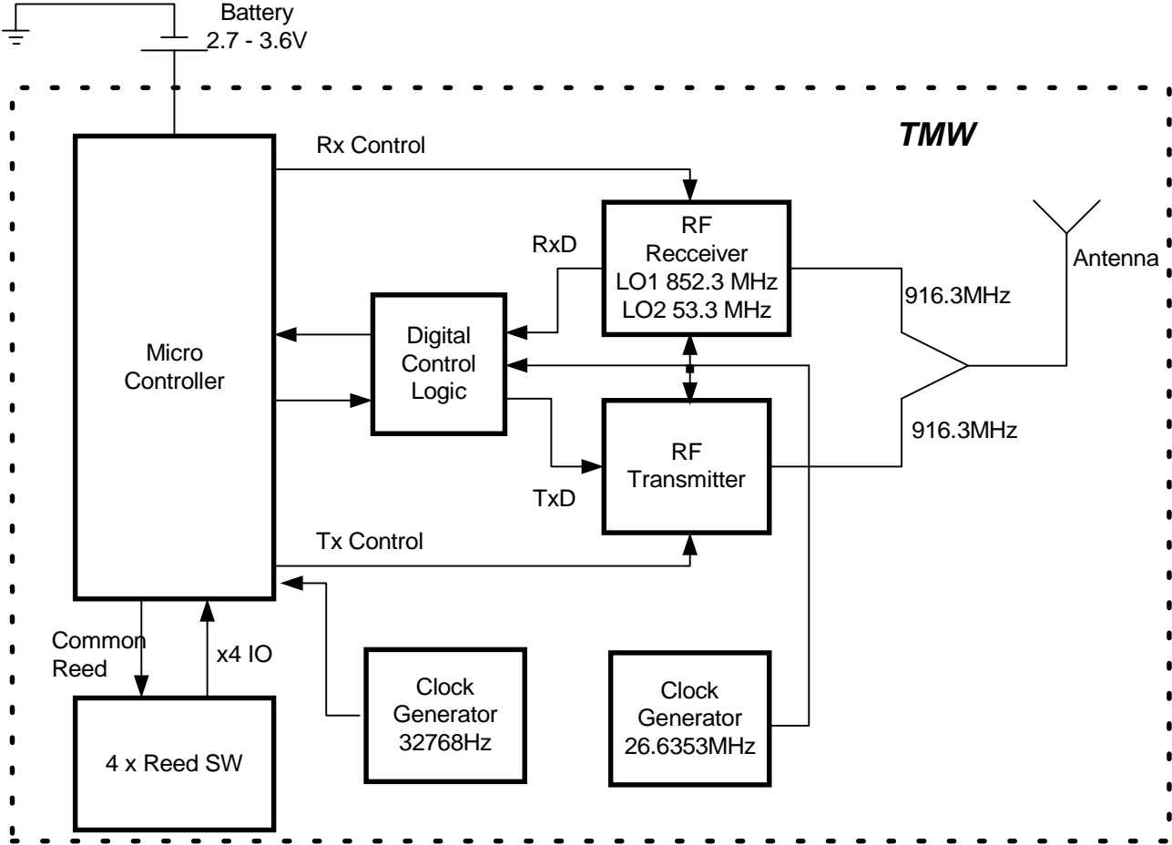
Figure 1: TMW Block Diagram
