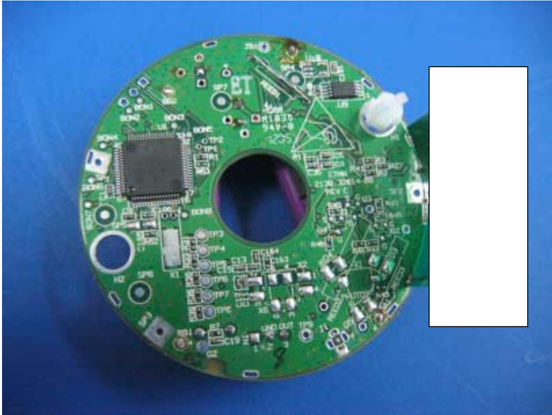
Photograph No.4 ETMW-NA water reader PCB printed side
