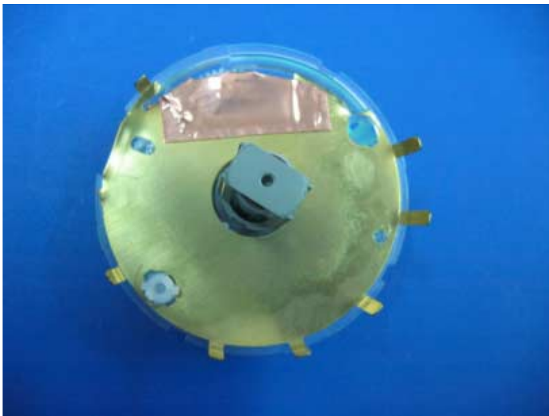
Photograph No.1 ETMW-NA water reader Shield separating water reader mechanical part from radio part
