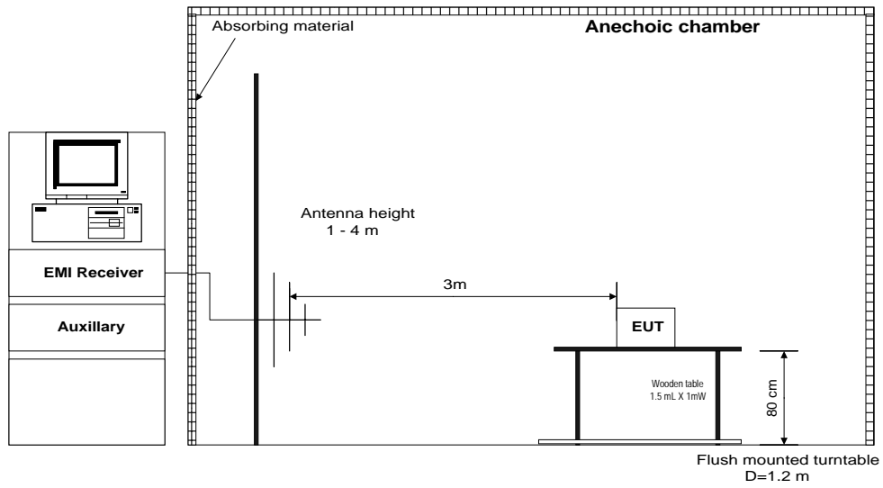
Figure 4.1.1 Setup for radiated emissions test, anechoic chamber method
