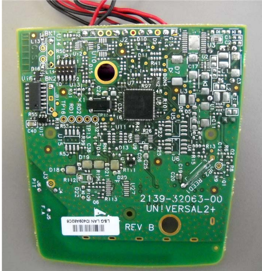
Photograph No.4 PCB second side close view
