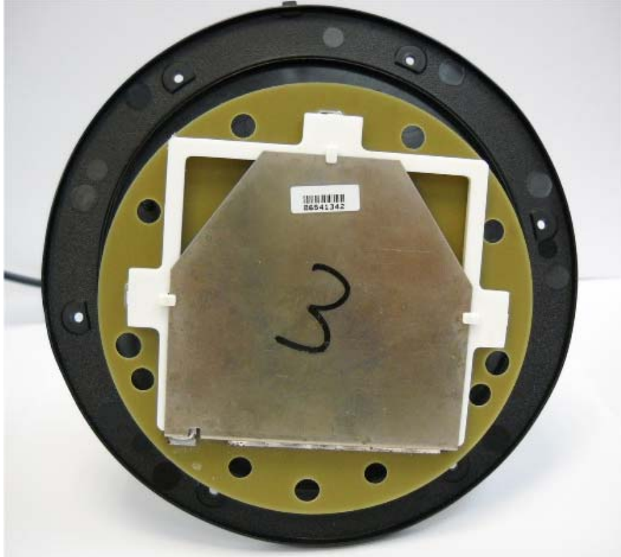
Photograph No.7 2WB-LG booster antenna
