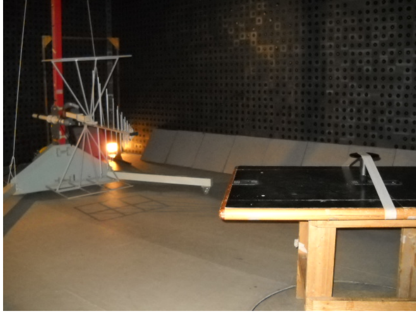
Photograph No.1 Setup for carrier field strength and power spectral density measurements in the anechoic chamber from 30 to 1000 MHz
