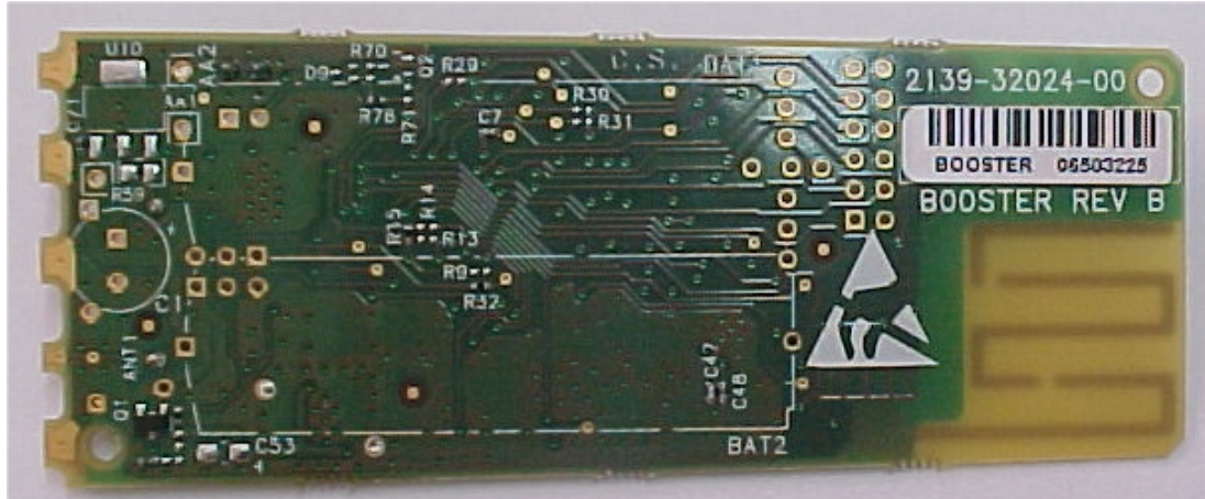
Photograph No.9 Booster water meter PCB
