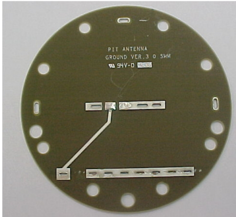
Photograph No.12 Booster water meter external antenna PCB
