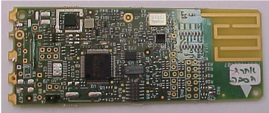
Photograph No.10 Booster water meter PCB, second side
