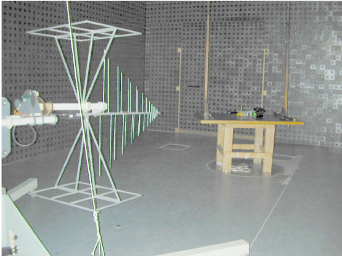
Photograph 4.1.1 Setup for radiated emission measurements 30 MHz – 1 GHz
