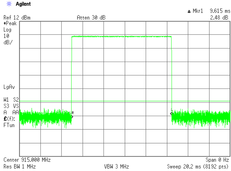
Plot 7.3.13 Transmission pulse duration
