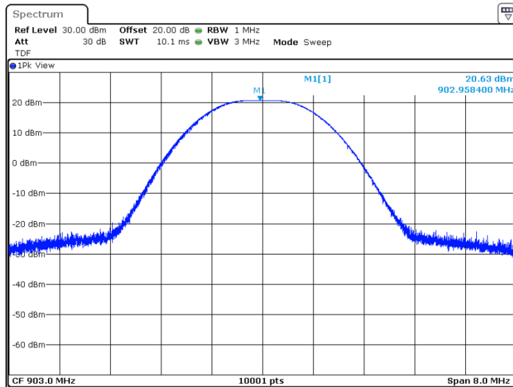
Plot 7.2.1 Peak output power at low frequency and Unom
