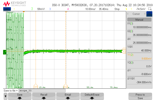
Plot 7.6.3 Transient frequency during power ON test results at mid carrier frequency
