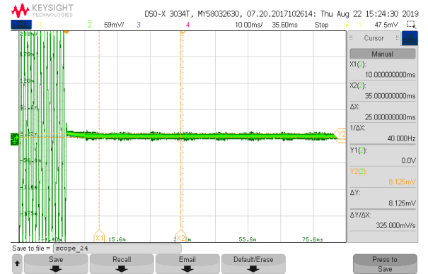
Plot 7.6.1 Transient frequency during power ON test results at low carrier frequency
