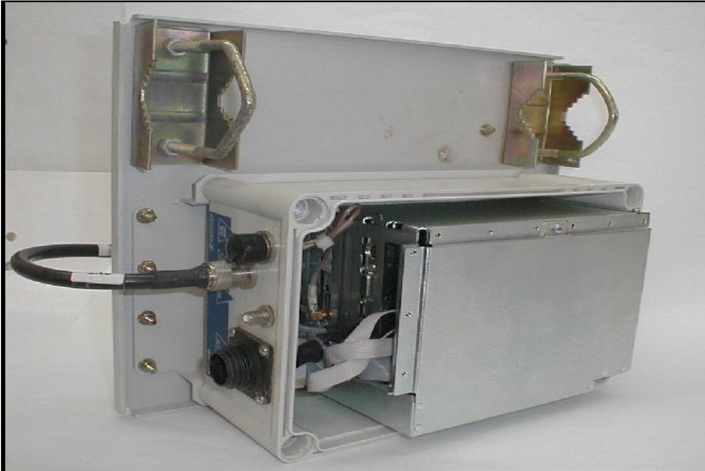
RSC-900 open
