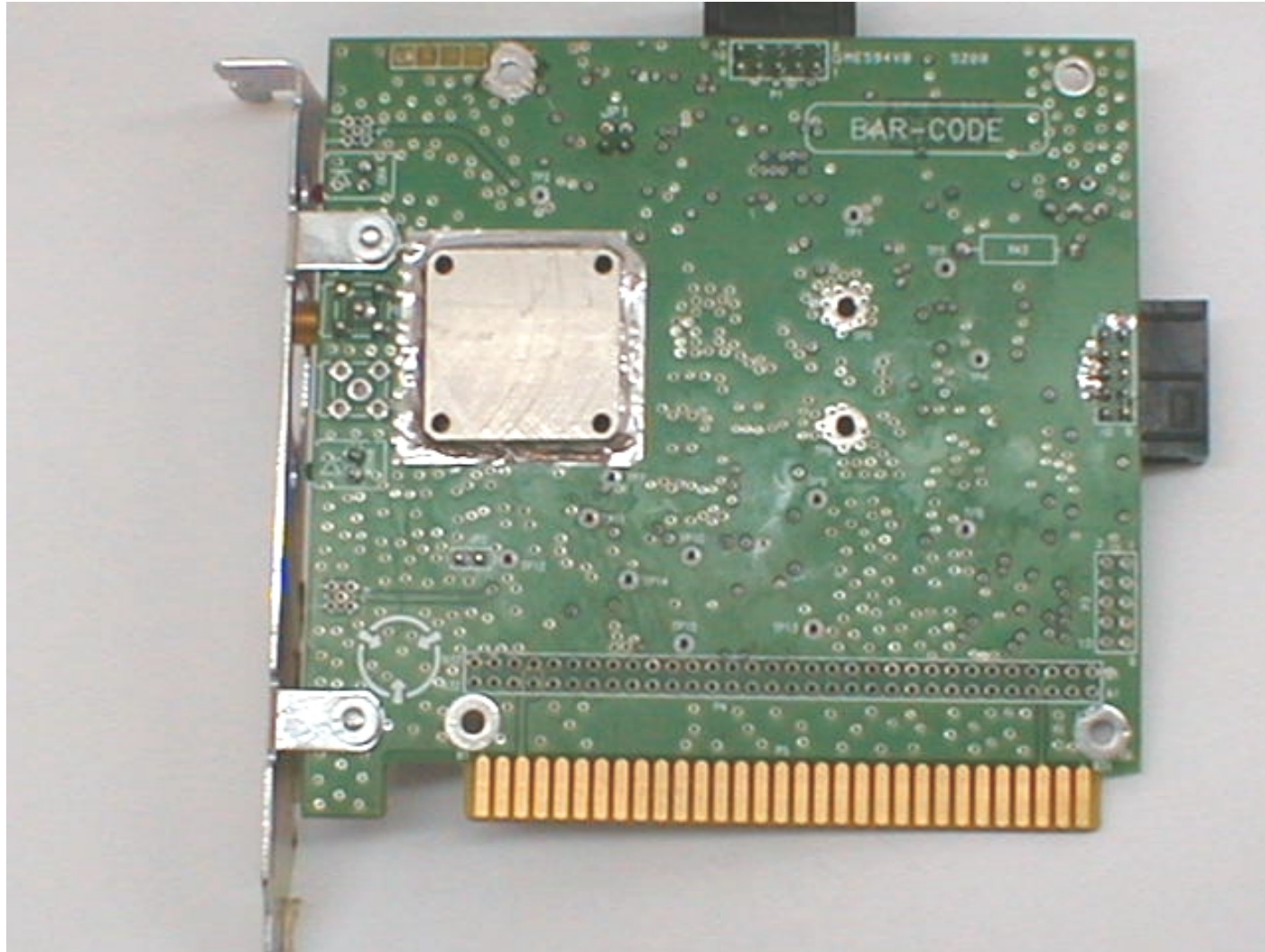
RFU printed side
