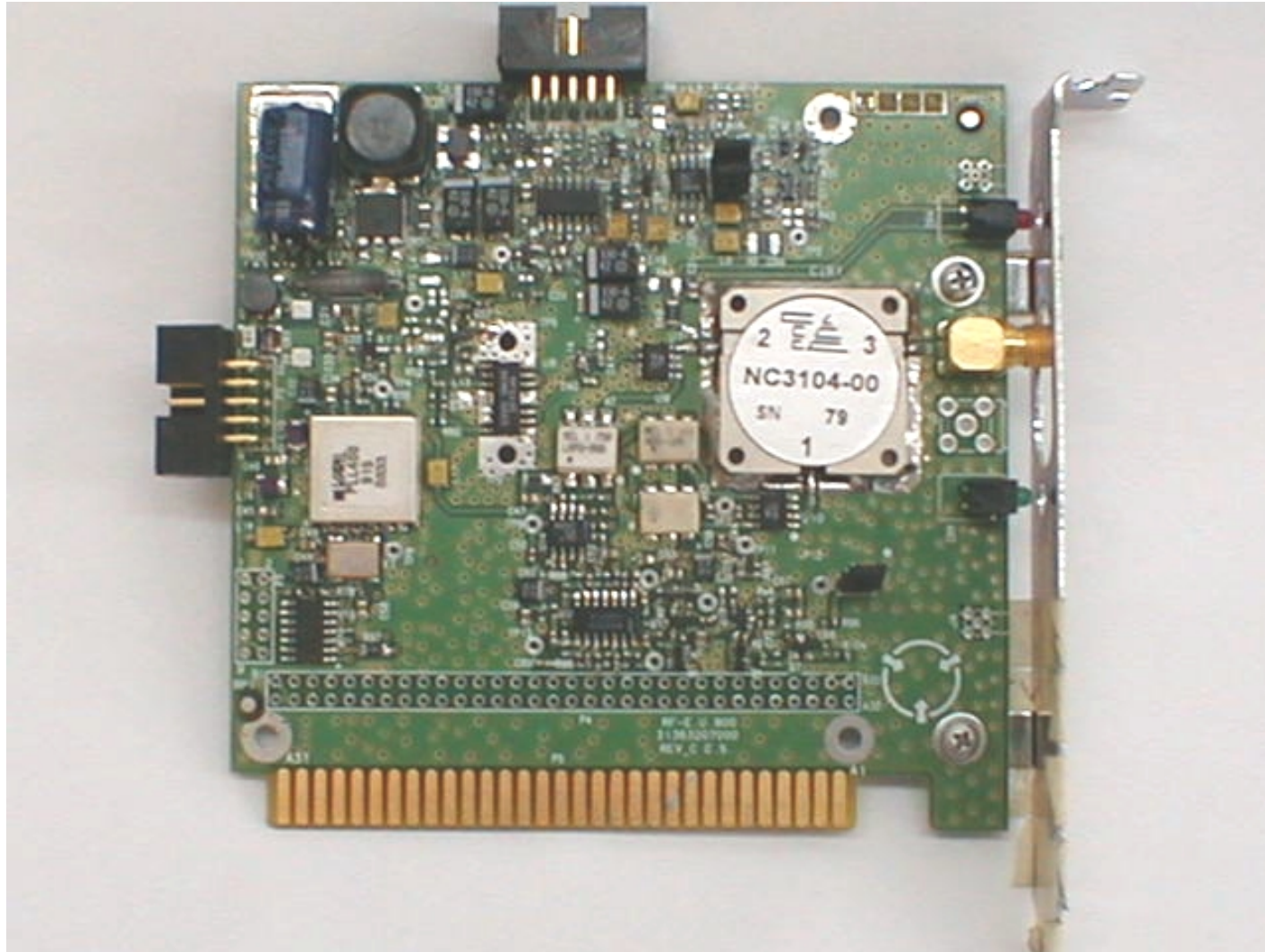
RFU component side
