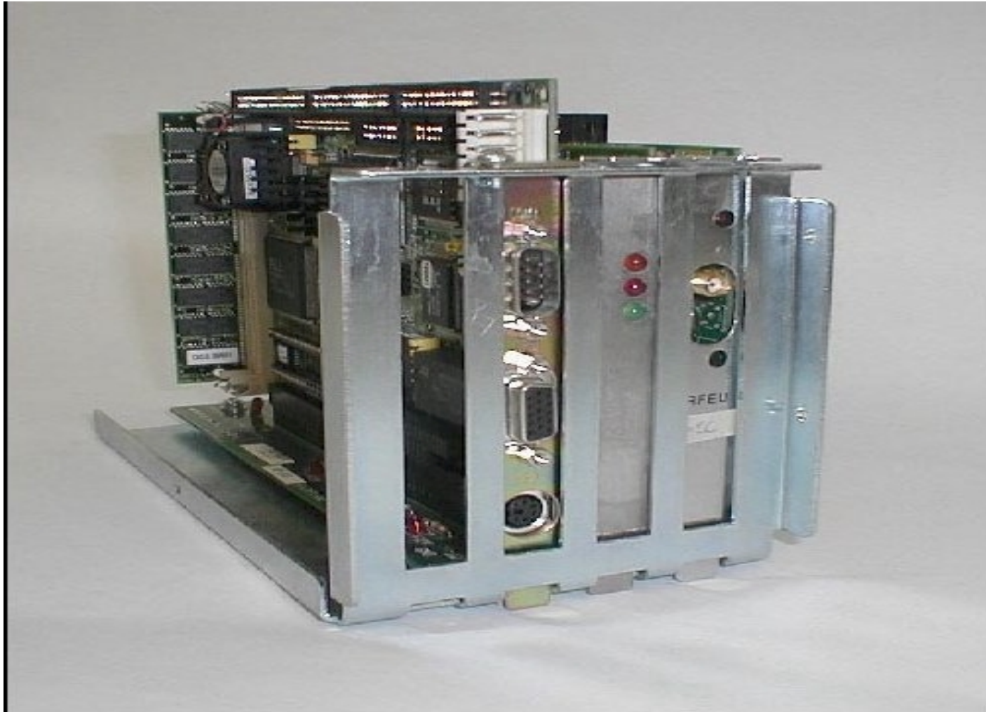
RSC-900 boards
