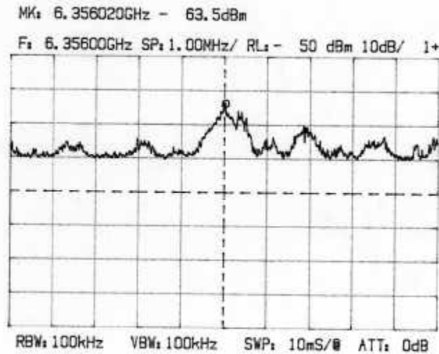
Plot 4.5.18 7 th harmonic, location transmission mode
