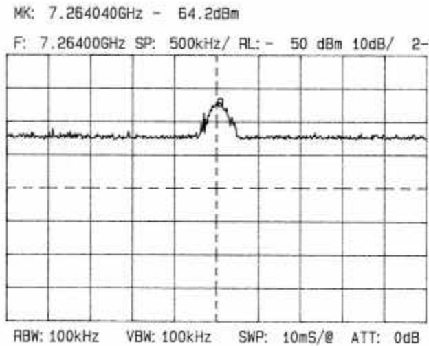
Plot 4.5.36 8 th harmonic, ECM transmission mode
