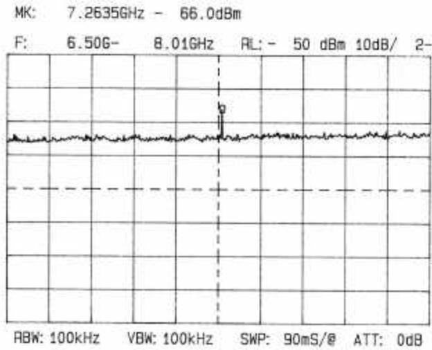
Plot 4.5.35 Frequency range 6.5 – 8 GHz, ECM transmission mode
