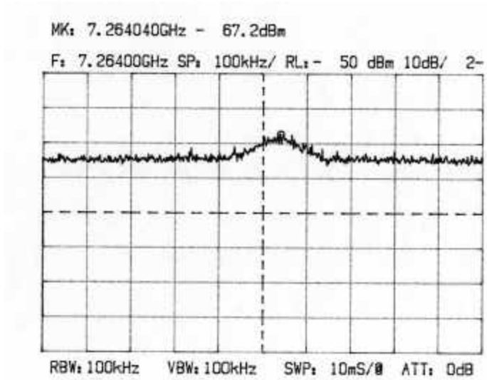
Plot 4.5.19 8 th harmonic, location transmission mode
