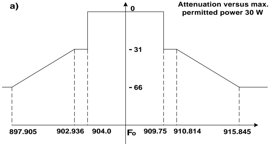
Figure 4.5.2 Emission mask ( F_0 = 906.875 MHz), ECM transmission mode
