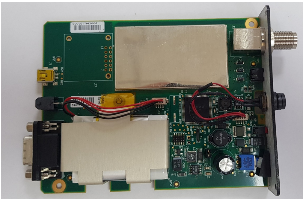
PCB top with RF shield
