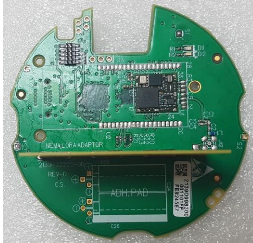
Photograph No.4 Component side of the RF PCB
