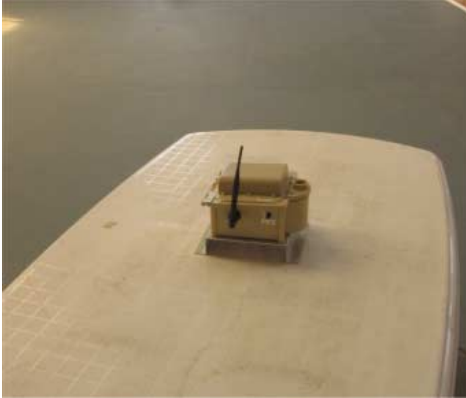
Photograph No.7 Spurious radiated emissions measurement setup at the OATS, EUT close view
