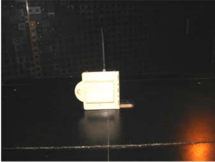
Photograph No.5 Radiated emissions measurement setup in the anechoic chamber close view
