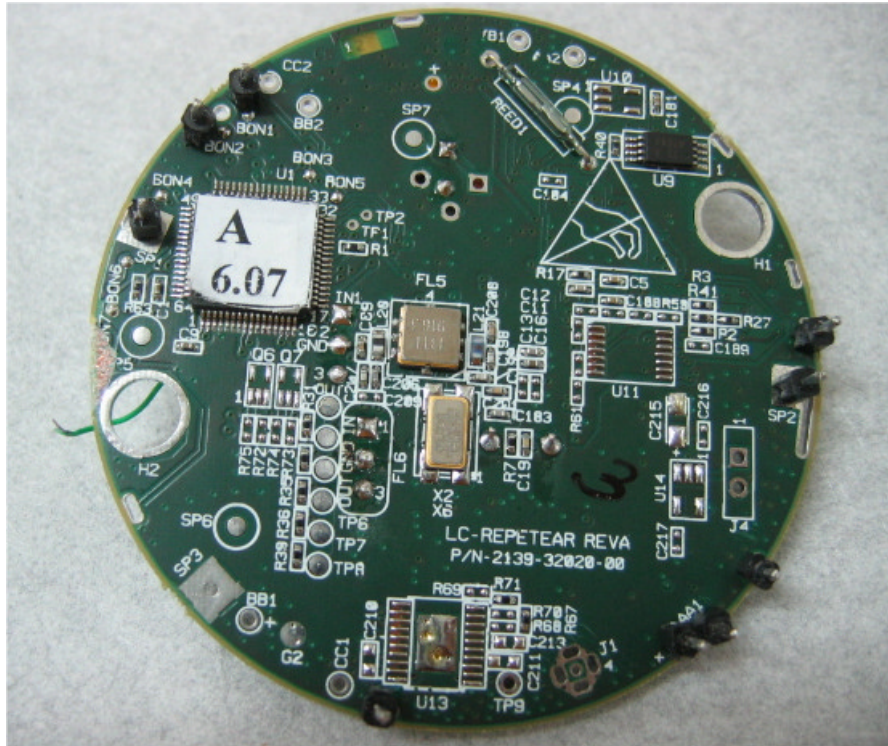
Photograph No.8 RF PCB second side view
