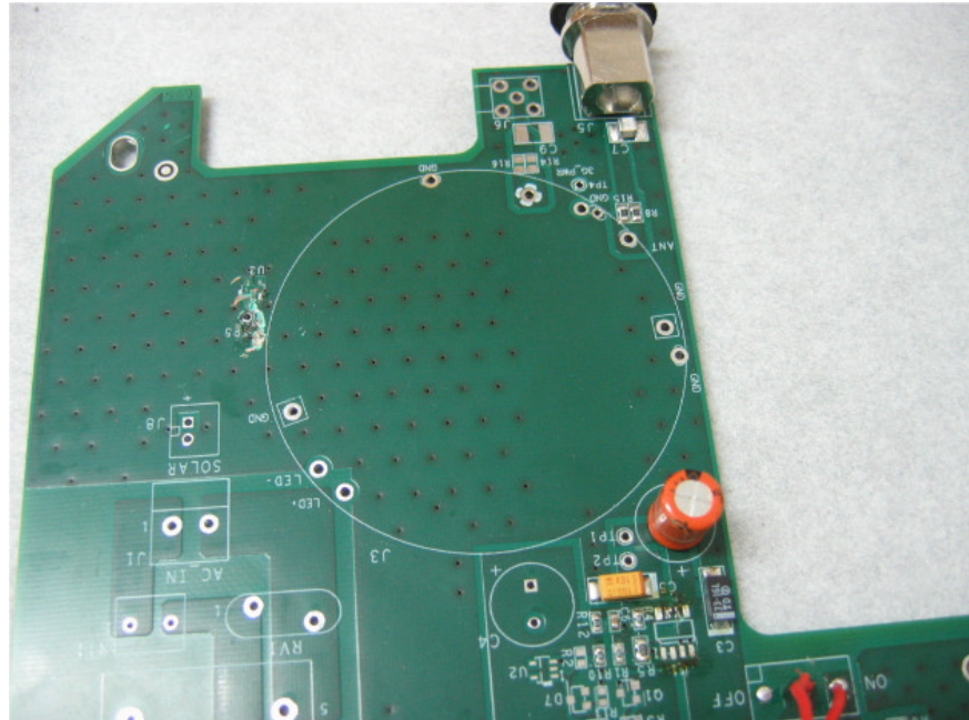
Photograph No.9 LCR main PCB component side with RF module
