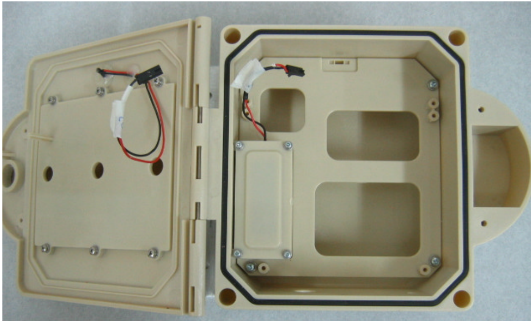
Photograph No.3 Low cost repeater (LCR) with PCB removed
