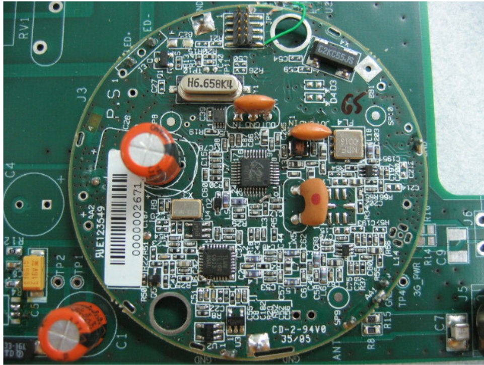
Photograph No.6 RF module close view
