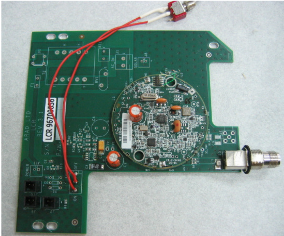
Photograph No.4 LCR main PCB component side with RF module
