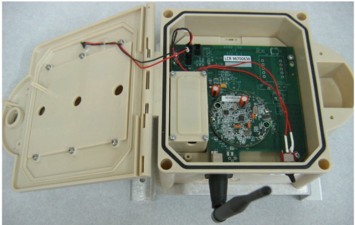
Photograph No.1 Low cost repeater (LCR) Internal view
