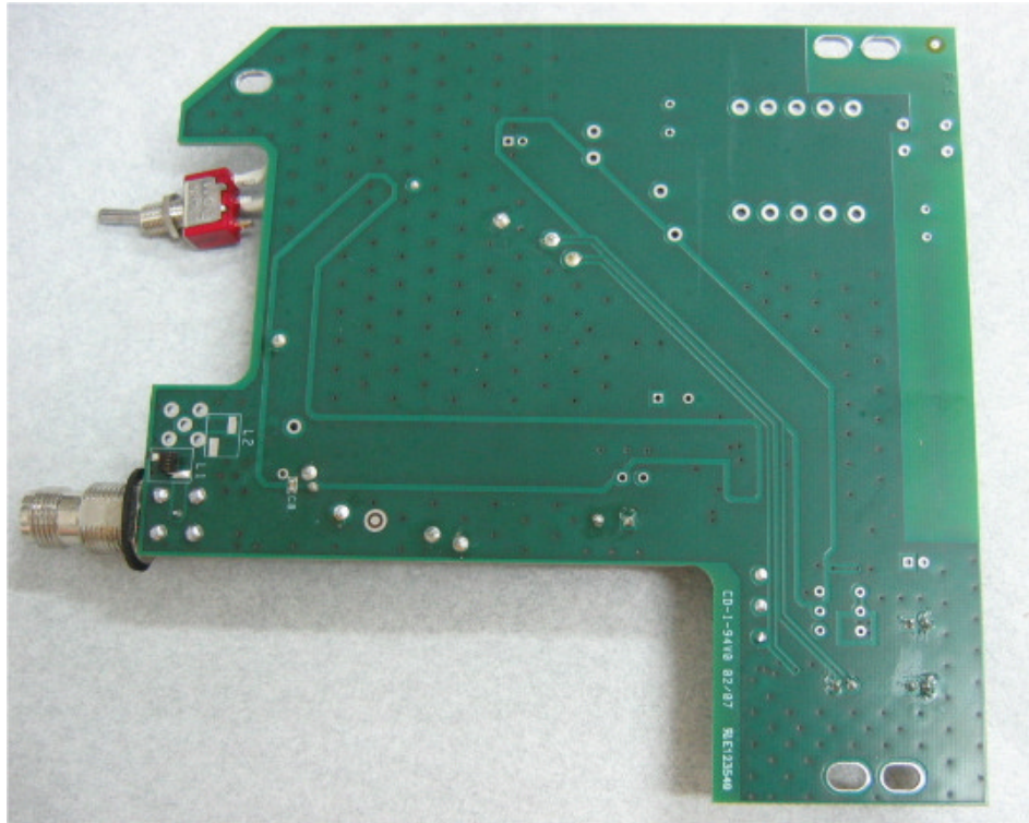
Photograph No.5 LCR main PCB second side view
