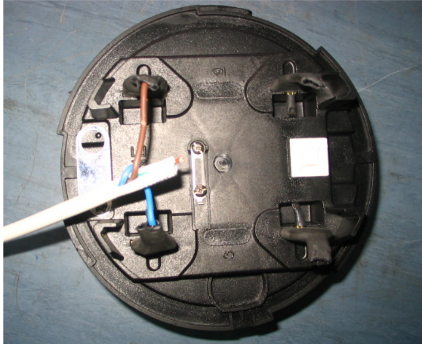
Photograph No.2 ICON240V electricity meter bottom view
