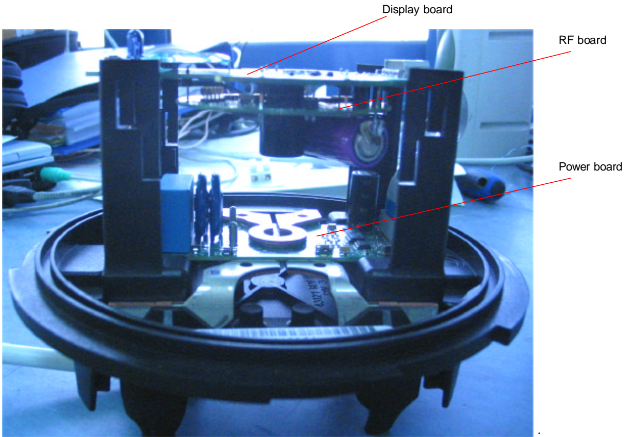
Photograph No.2 ICON240V meter side view
