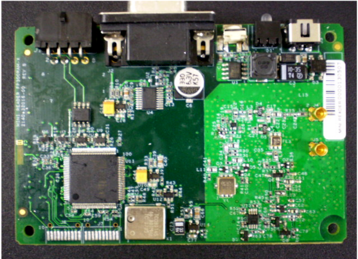
Photograph No.3 Roadside mini reader PCB upper view
