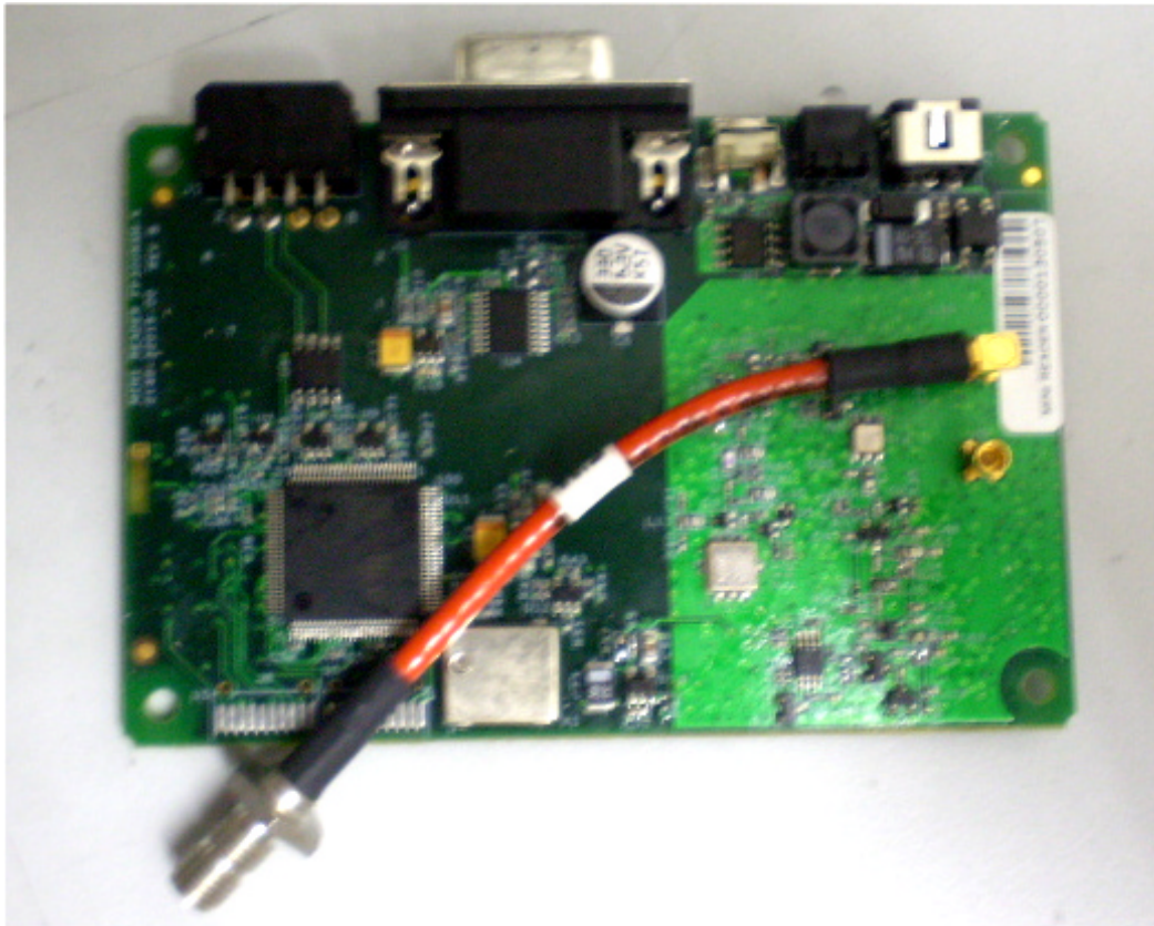
Photograph No.2 Roadside mini reader PCB with antenna assembly
