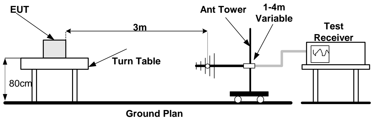
Figure 5.f Radiated Emission Set up
