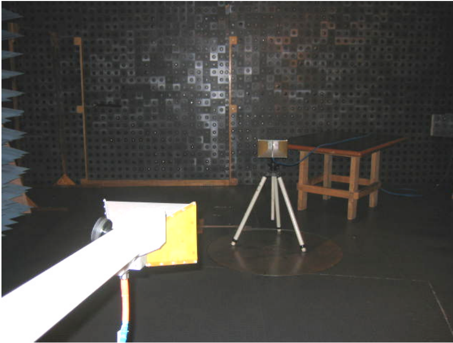
Photograph No.8 Substitution ERP measurement of spurious setup in the anechoic chamber
