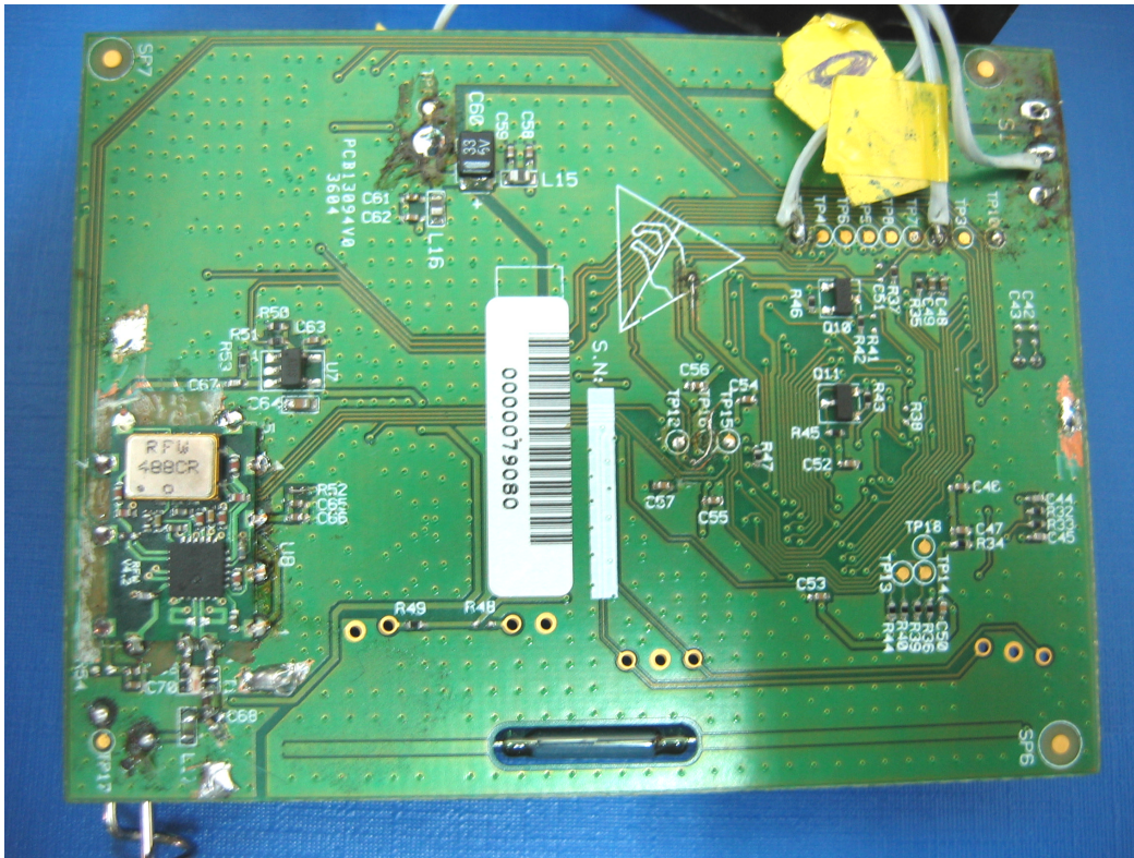
Photograph No.4 FP200INT electronic seal PCB second side view
