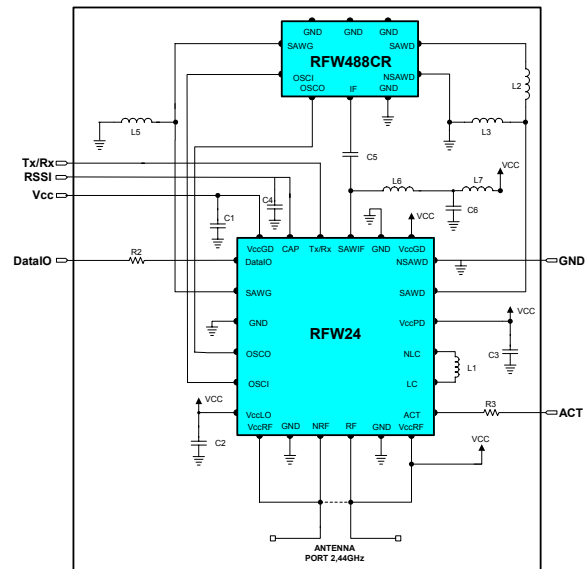
Figure 2: Transceiver Implementation - Using RFW112 Chipset
