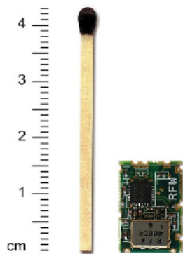
Figure 1: Actual Size of a Typical Transceiver Using RFW112 Chipset
