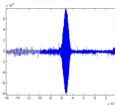
Figure 7: Autocorrelation
